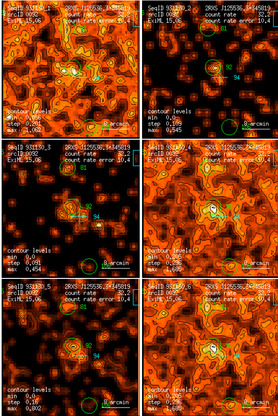
Figure 92: RASS 931130: detection 0092: band rate images, Gaussian filter: (1) PSPC channels 11 – 41, (2) 52 – 90, (3) 91 – 201, (4) 11 – 235, (5) 52 – 201, (6) 11 – 201. Broad band rates in counts/ks. Band rate contour levels in counts/ks/arcmin 2 .
