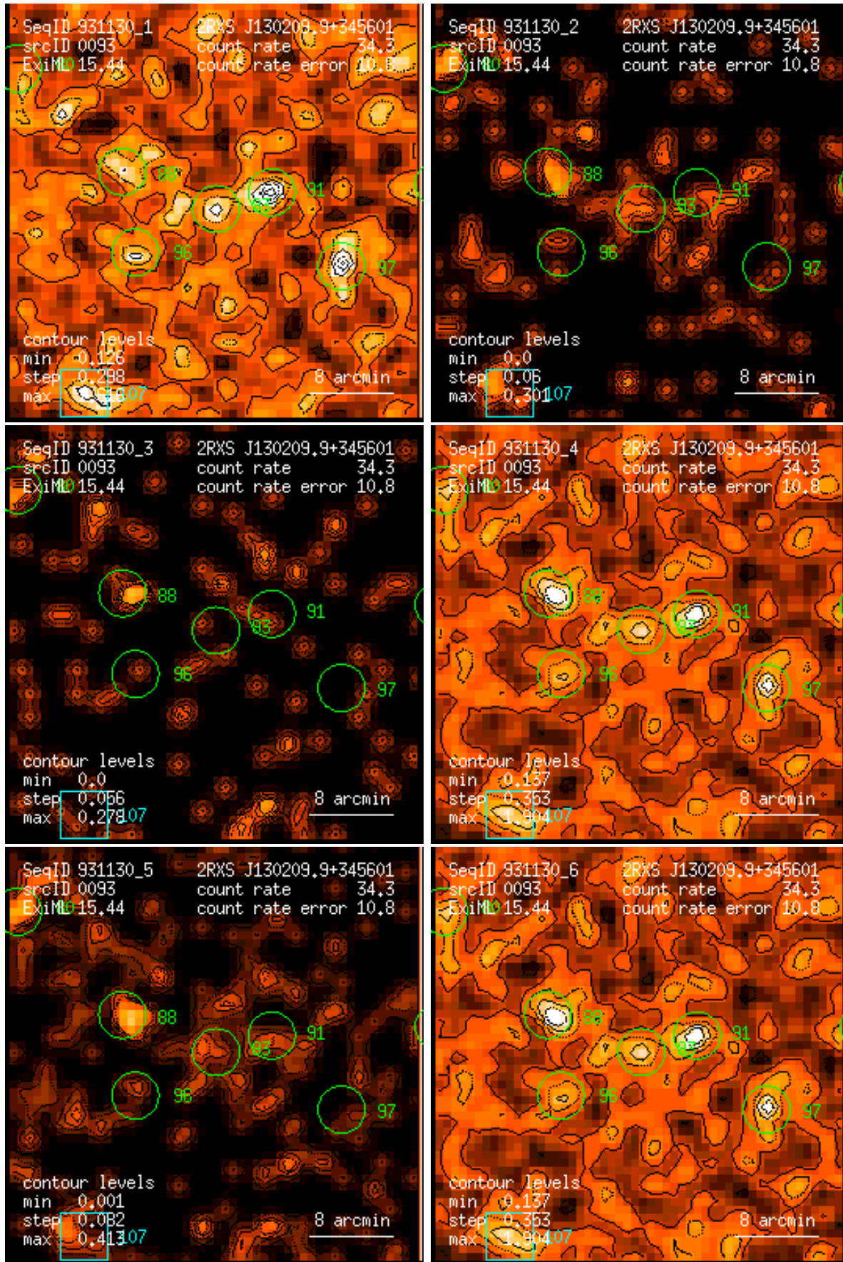
Figure 93: RASS 931130: detection 0093: band rate images, Gaussian filter: (1) PSPC channels 11 – 41, (2) 52 – 90, (3) 91 – 201, (4) 11 – 235, (5) 52 – 201, (6) 11 – 201. Broad band rates in counts/ks. Band rate contour levels in counts/ks/arcmin 2 .
