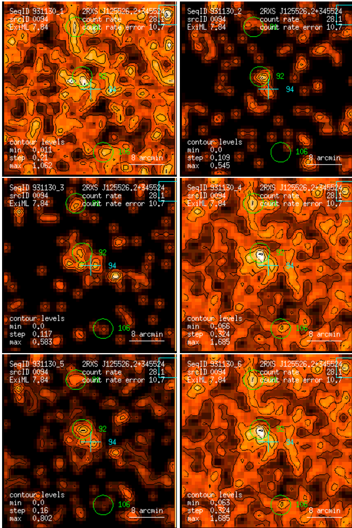
Figure 94: RASS 931130: detection 0094: band rate images, Gaussian filter: (1) PSPC channels 11 – 41, (2) 52 – 90, (3) 91 – 201, (4) 11 – 235, (5) 52 – 201, (6) 11 – 201. Broad band rates in counts/ks. Band rate contour levels in counts/ks/arcmin 2 .
