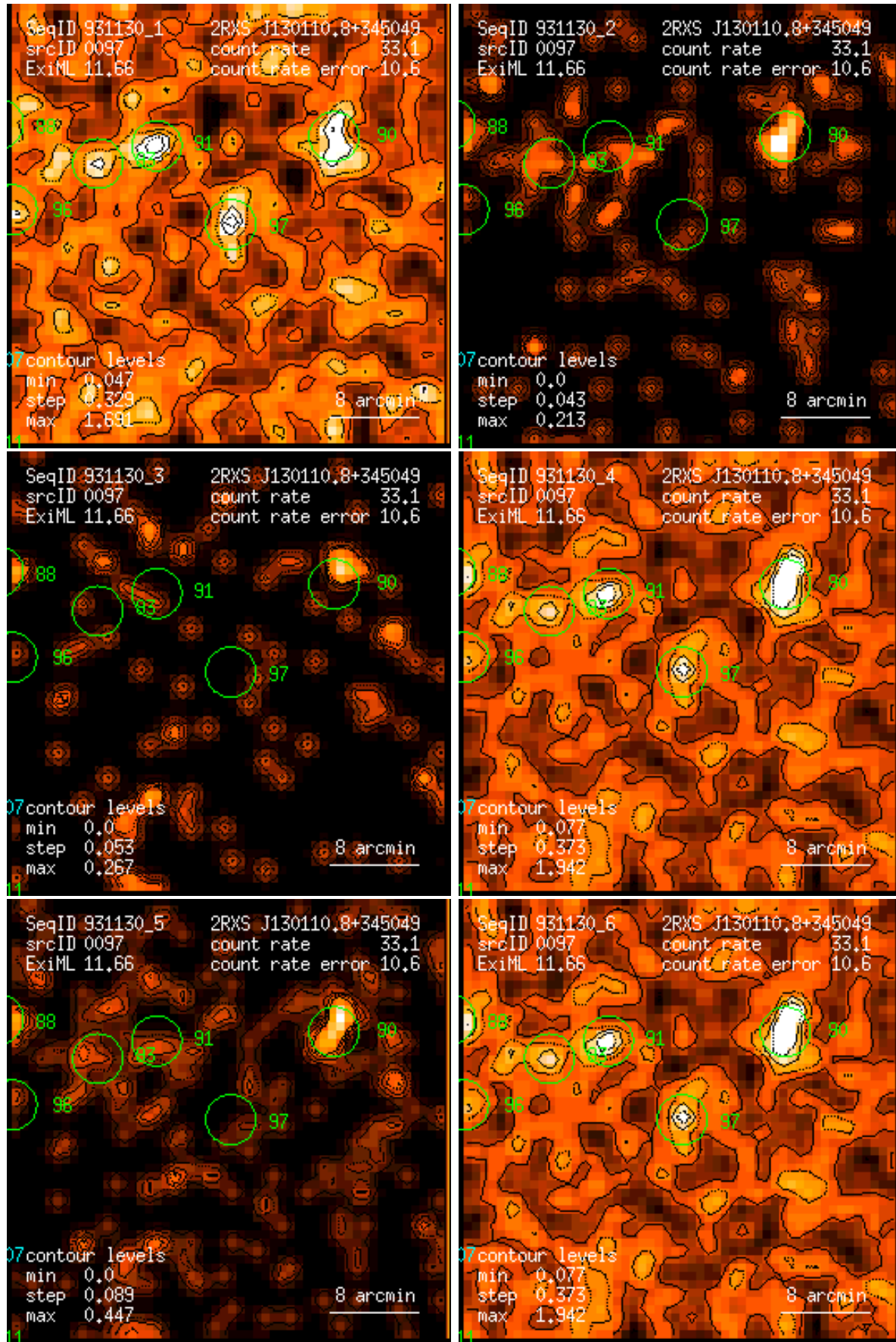
Figure 97: RASS 931130: detection 0097: band rate images, Gaussian filter: (1) PSPC channels 11 – 41, (2) 52 – 90, (3) 91 – 201, (4) 11 – 235, (5) 52 – 201, (6) 11 – 201. Broad band rates in counts/ks. Band rate contour levels in counts/ks/arcmin 2 .
