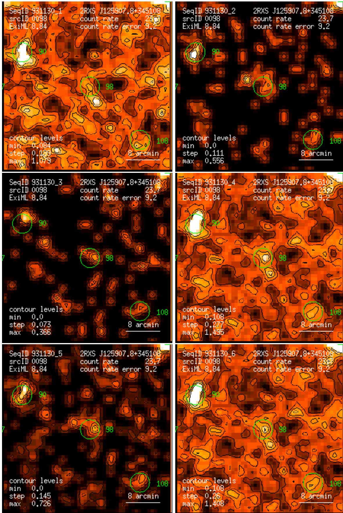
Figure 98: RASS 931130: detection 0098: band rate images, Gaussian filter: (1) PSPC channels 11 – 41, (2) 52 – 90, (3) 91 – 201, (4) 11 – 235, (5) 52 – 201, (6) 11 – 201. Broad band rates in counts/ks. Band rate contour levels in counts/ks/arcmin 2 .
