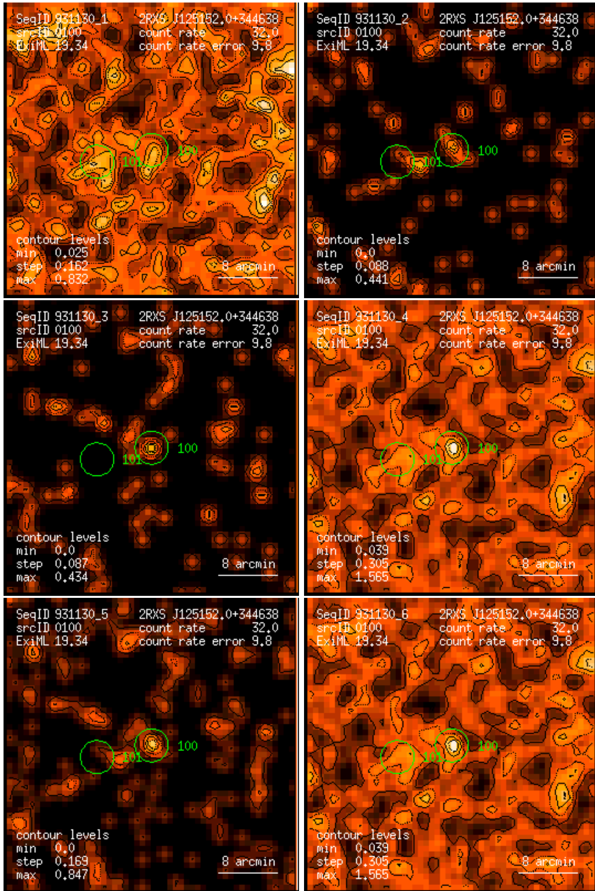
Figure 100: RASS 931130: detection 0100: band rate images, Gaussian filter: (1) PSPC channels 11 – 41, (2) 52 – 90, (3) 91 – 201, (4) 11 – 235, (5) 52 – 201, (6) 11 – 201. Broad band rates in counts/ks. Band rate contour levels in counts/ks/arcmin 2 .
