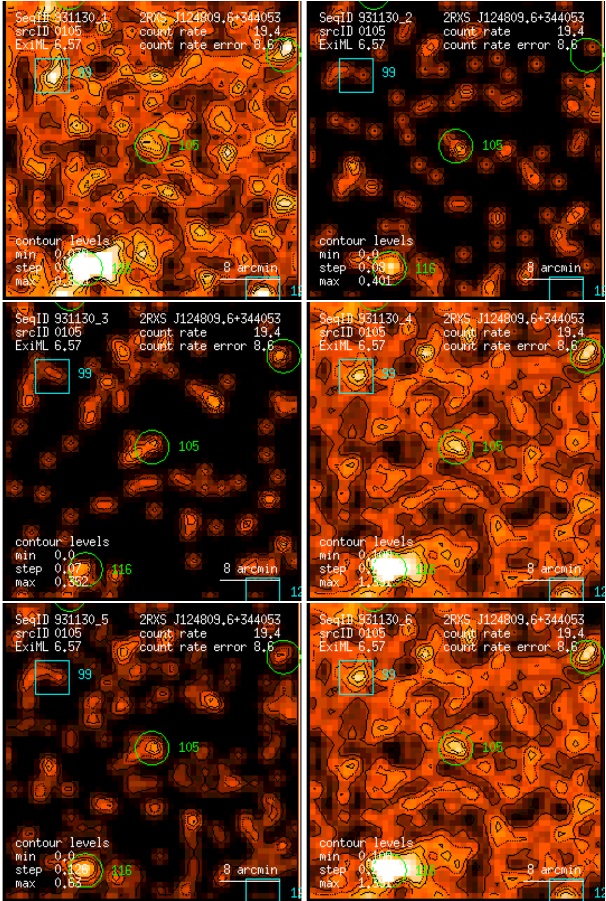
Figure 105: RASS 931130: detection 0105: band rate images, Gaussian filter: (1) PSPC channels 11 – 41, (2) 52 – 90, (3) 91 – 201, (4) 11 – 235, (5) 52 – 201, (6) 11 – 201. Broad band rates in counts/ks. Band rate contour levels in counts/ks/arcmin 2 .
