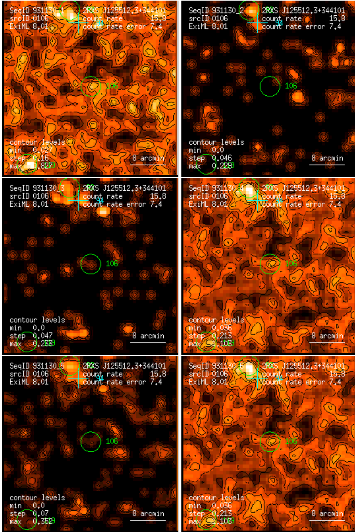
Figure 106: RASS 931130: detection 0106: band rate images, Gaussian filter: (1) PSPC channels 11 – 41, (2) 52 – 90, (3) 91 – 201, (4) 11 – 235, (5) 52 – 201, (6) 11 – 201. Broad band rates in counts/ks. Band rate contour levels in counts/ks/arcmin 2 .
