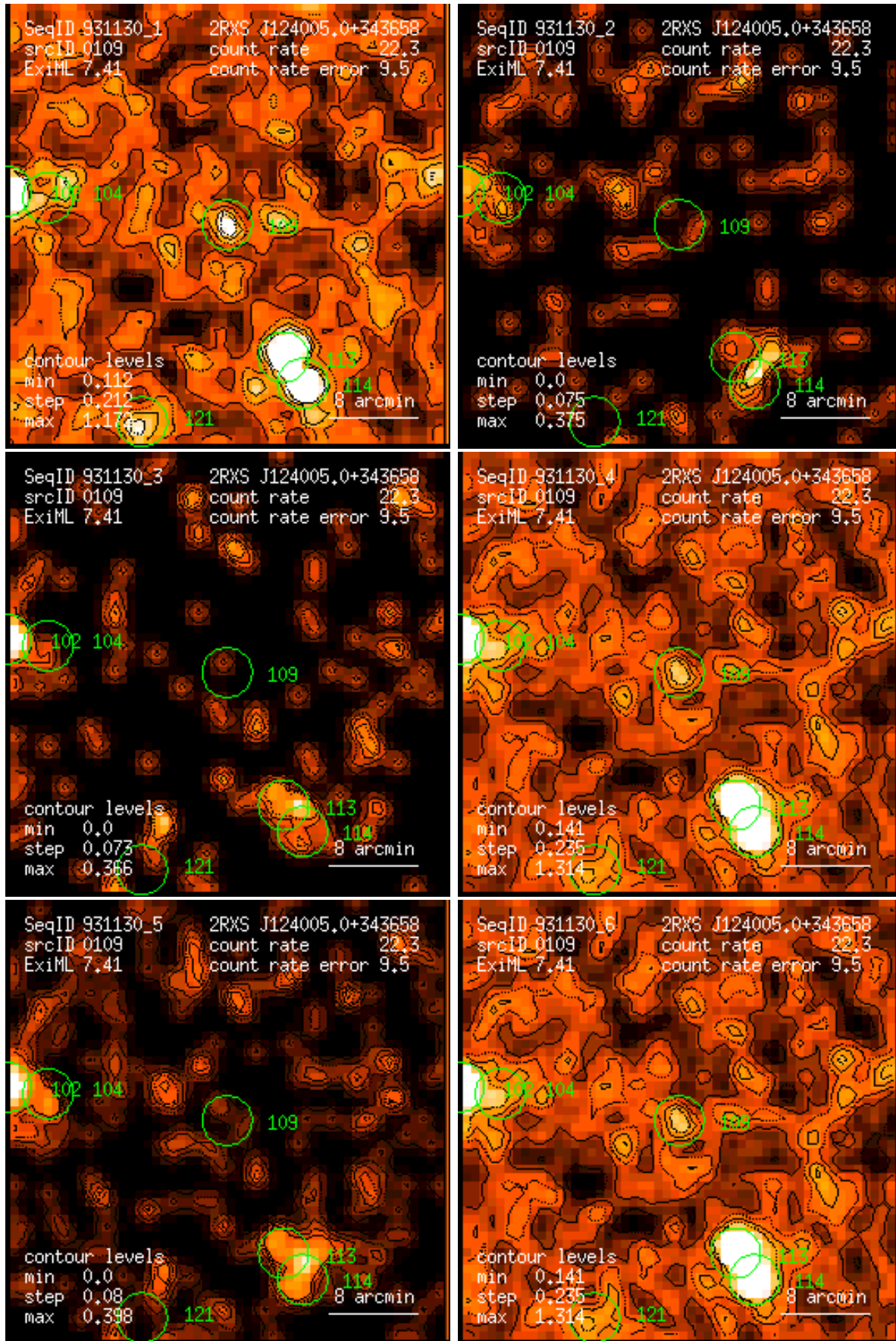
Figure 109: RASS 931130: detection 0109: band rate images, Gaussian filter: (1) PSPC channels 11 – 41, (2) 52 – 90, (3) 91 – 201, (4) 11 – 235, (5) 52 – 201, (6) 11 – 201. Broad band rates in counts/ks. Band rate contour levels in counts/ks/arcmin 2 .
