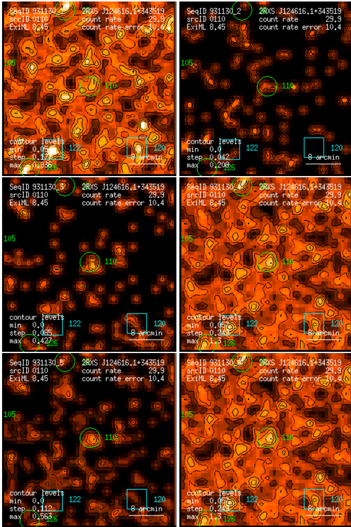
Figure 110: RASS 931130: detection 0110: band rate images, Gaussian filter: (1) PSPC channels 11 – 41, (2) 52 – 90, (3) 91 – 201, (4) 11 – 235, (5) 52 – 201, (6) 11 – 201. Broad band rates in counts/ks. Band rate contour levels in counts/ks/arcmin 2 .
