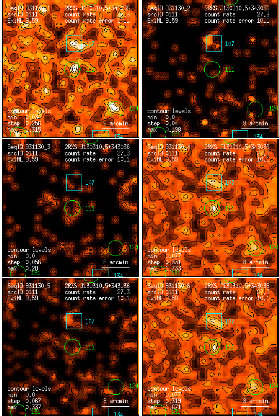
Figure 111: RASS 931130: detection 0111: band rate images, Gaussian filter: (1) PSPC channels 11 – 41, (2) 52 – 90, (3) 91 – 201, (4) 11 – 235, (5) 52 – 201, (6) 11 – 201. Broad band rates in counts/ks. Band rate contour levels in counts/ks/arcmin 2 .
