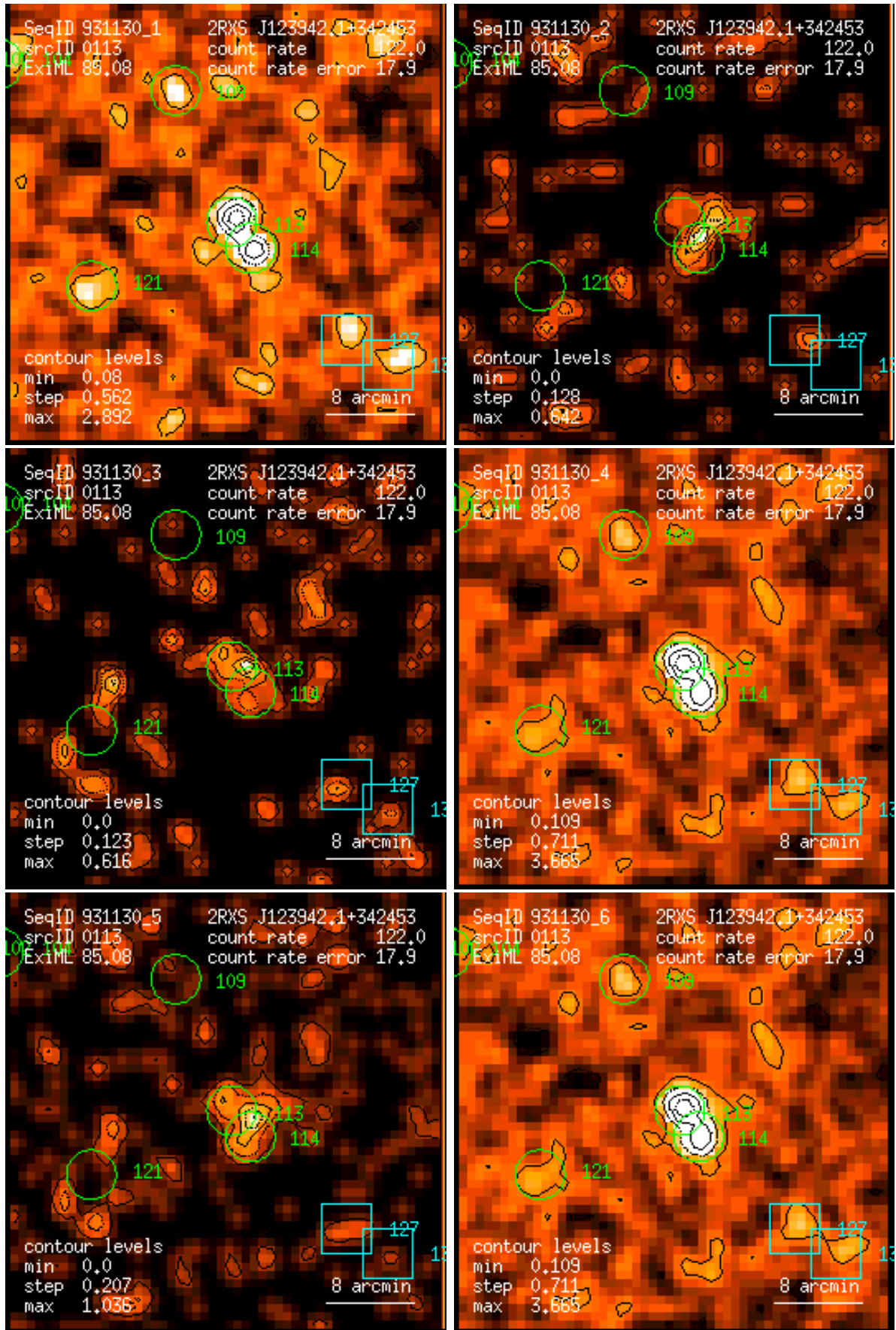
Figure 113: RASS 931130: detection 0113: band rate images, Gaussian filter: (1) PSPC channels 11 – 41, (2) 52 – 90, (3) 91 – 201, (4) 11 – 235, (5) 52 – 201, (6) 11 – 201. Broad band rates in counts/ks. Band rate contour levels in counts/ks/arcmin 2 .
