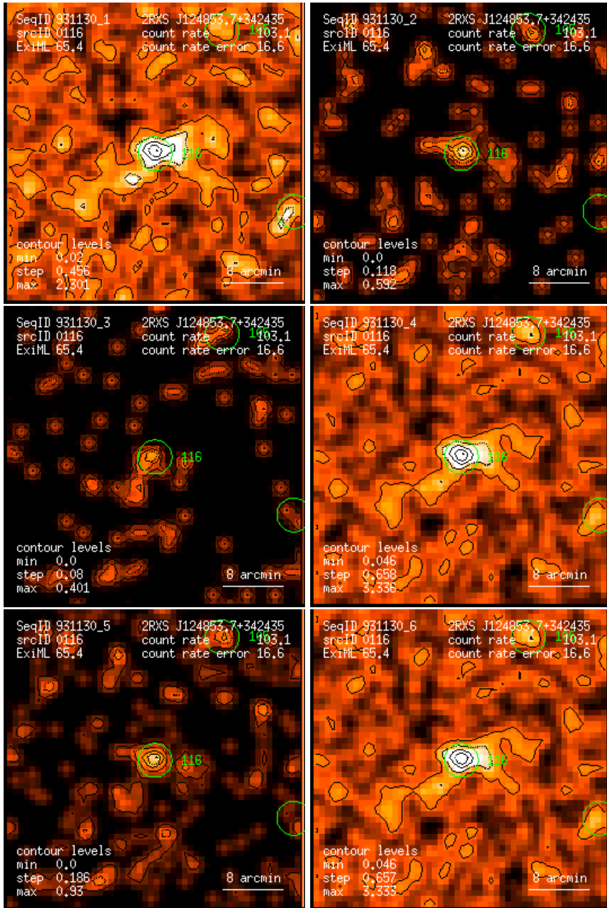
Figure 116: RASS 931130: detection 0116: band rate images, Gaussian filter: (1) PSPC channels 11 – 41, (2) 52 – 90, (3) 91 – 201, (4) 11 – 235, (5) 52 – 201, (6) 11 – 201. Broad band rates in counts/ks. Band rate contour levels in counts/ks/arcmin 2 .
