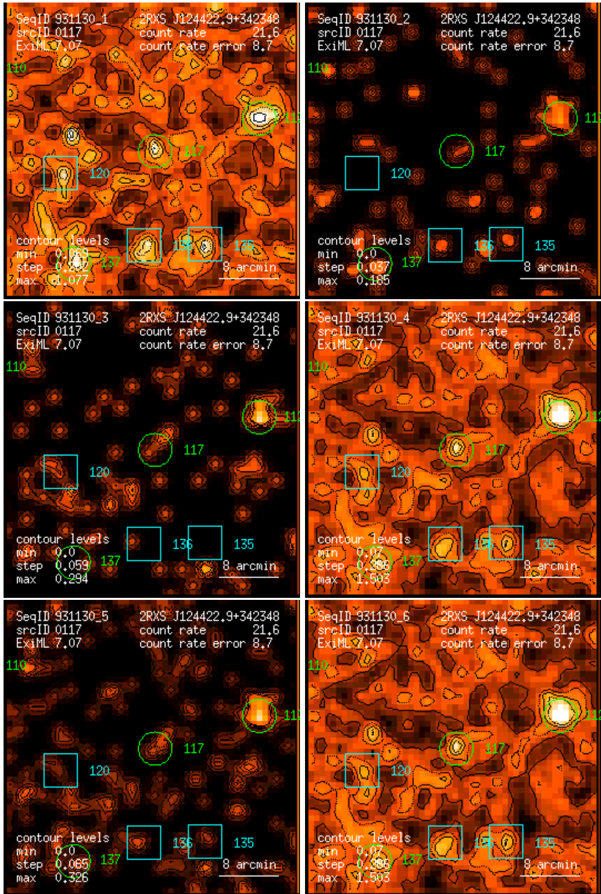
Figure 117: RASS 931130: detection 0117: band rate images, Gaussian filter: (1) PSPC channels 11 – 41, (2) 52 – 90, (3) 91 – 201, (4) 11 – 235, (5) 52 – 201, (6) 11 – 201. Broad band rates in counts/ks. Band rate contour levels in counts/ks/arcmin 2 .
