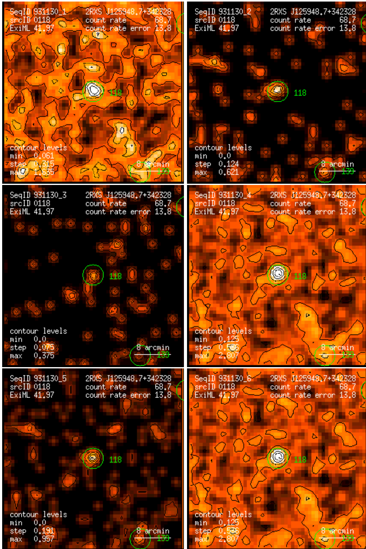
Figure 118: RASS 931130: detection 0118: band rate images, Gaussian filter: (1) PSPC channels 11 – 41, (2) 52 – 90, (3) 91 – 201, (4) 11 – 235, (5) 52 – 201, (6) 11 – 201. Broad band rates in counts/ks. Band rate contour levels in counts/ks/arcmin 2 .
