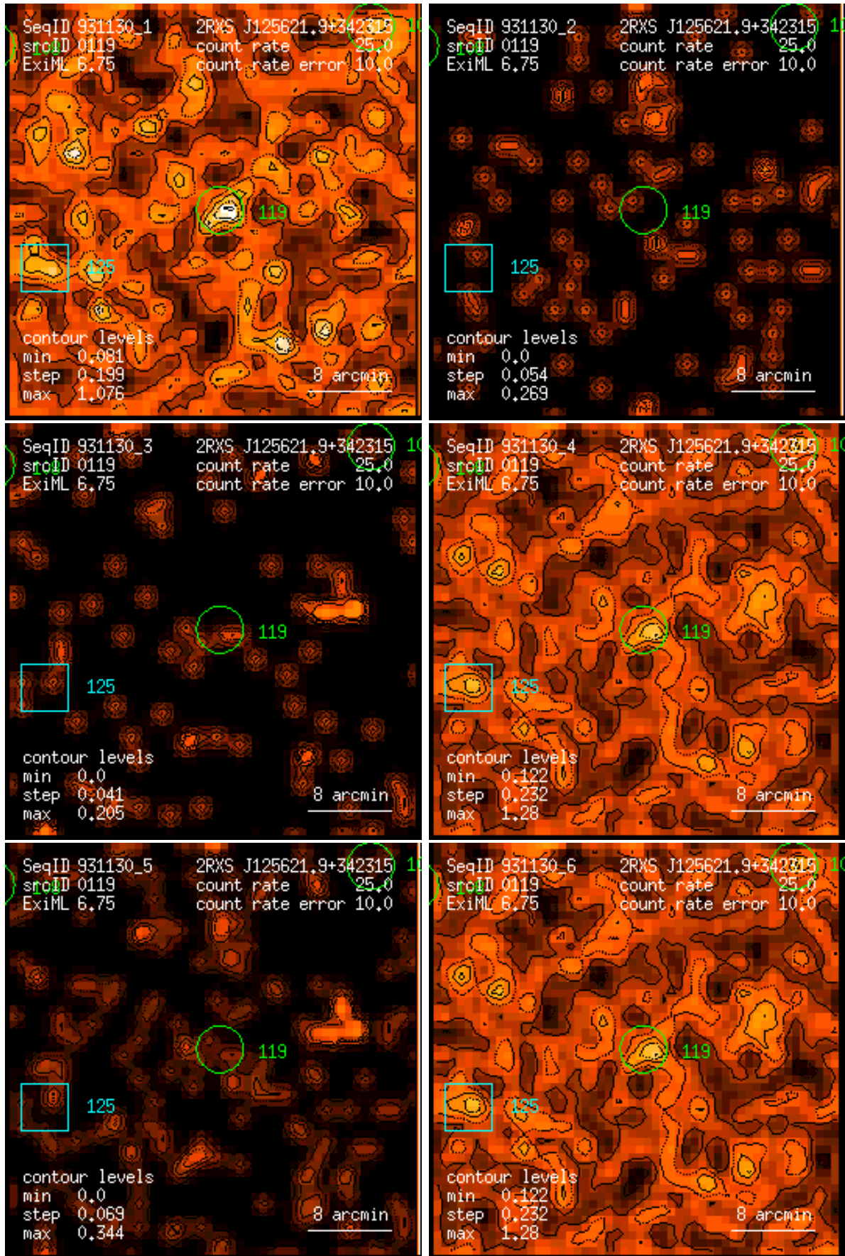
Figure 119: RASS 931130: detection 0119: band rate images, Gaussian filter: (1) PSPC channels 11 – 41, (2) 52 – 90, (3) 91 – 201, (4) 11 – 235, (5) 52 – 201, (6) 11 – 201. Broad band rates in counts/ks. Band rate contour levels in counts/ks/arcmin 2 .
