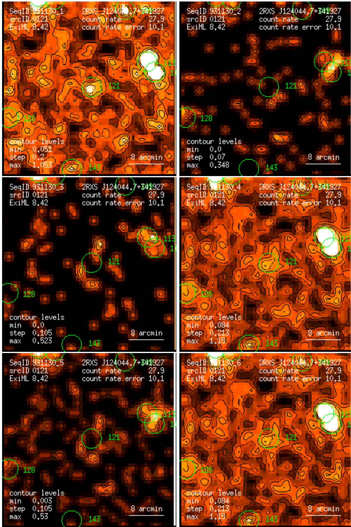
Figure 121: RASS 931130: detection 0121: band rate images, Gaussian filter: (1) PSPC channels 11 – 41, (2) 52 – 90, (3) 91 – 201, (4) 11 – 235, (5) 52 – 201, (6) 11 – 201. Broad band rates in counts/ks. Band rate contour levels in counts/ks/arcmin 2 .
