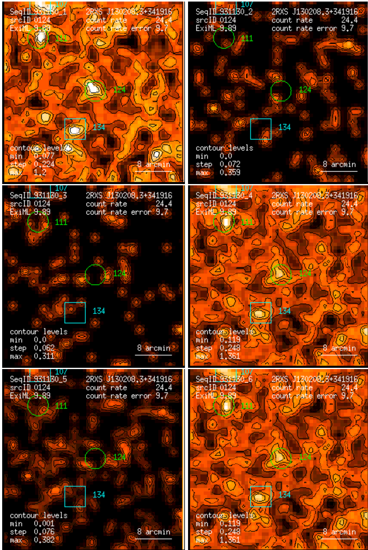
Figure 124: RASS 931130: detection 0124: band rate images, Gaussian filter: (1) PSPC channels 11 – 41, (2) 52 – 90, (3) 91 – 201, (4) 11 – 235, (5) 52 – 201, (6) 11 – 201. Broad band rates in counts/ks. Band rate contour levels in counts/ks/arcmin 2 .
