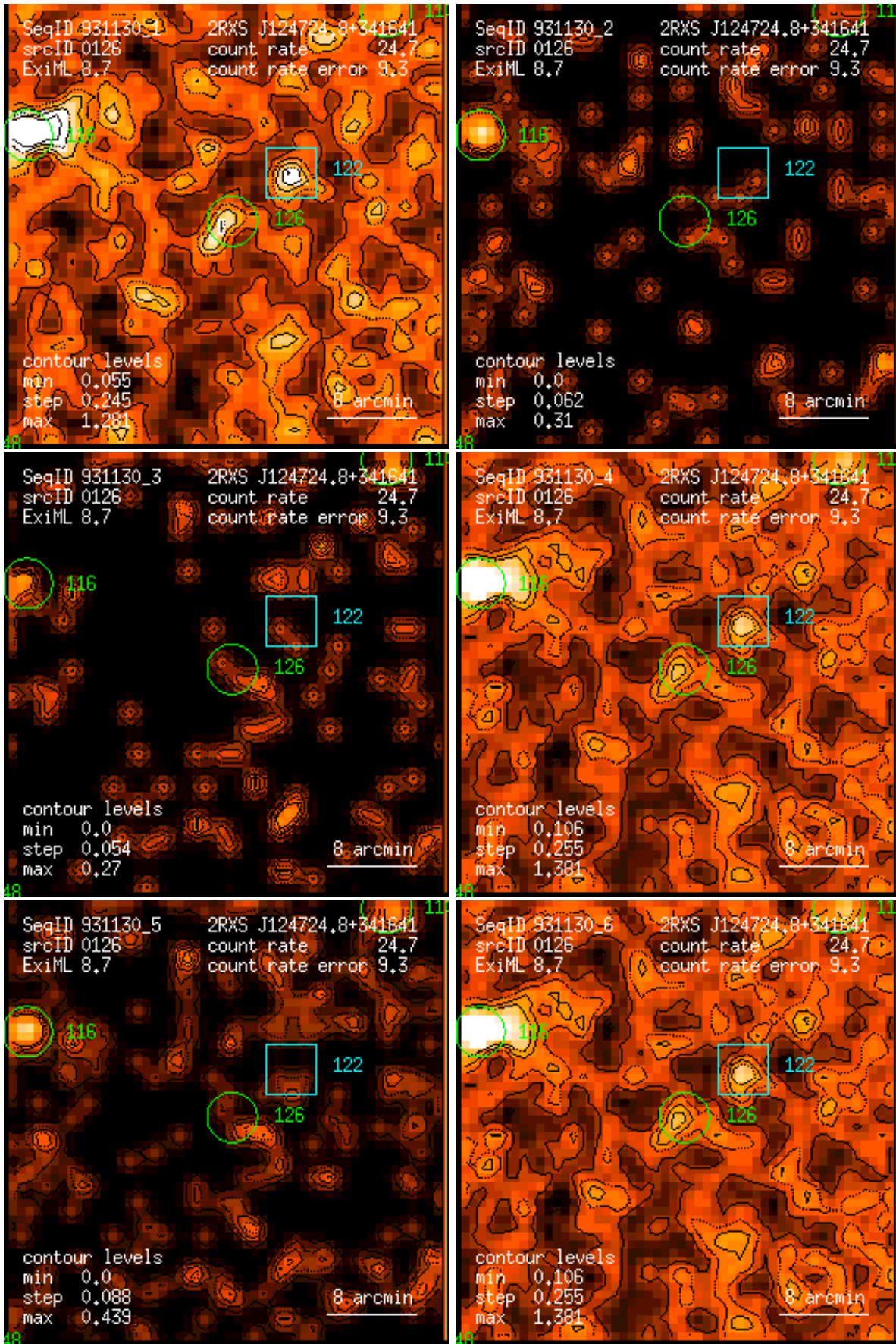
Figure 126: RASS 931130: detection 0126: band rate images, Gaussian filter: (1) PSPC channels 11 – 41, (2) 52 – 90, (3) 91 – 201, (4) 11 – 235, (5) 52 – 201, (6) 11 – 201. Broad band rates in counts/ks. Band rate contour levels in counts/ks/arcmin 2 .
