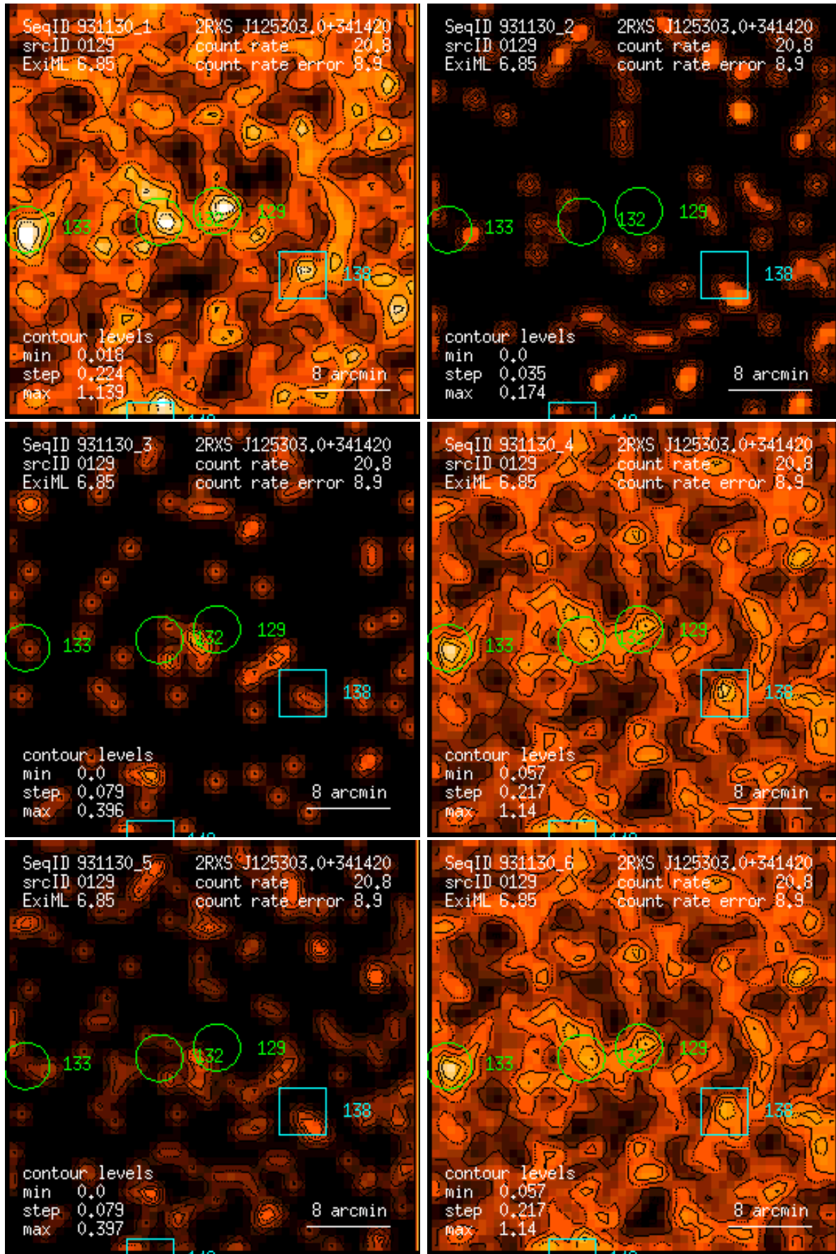
Figure 129: RASS 931130: detection 0129: band rate images, Gaussian filter: (1) PSPC channels 11 – 41, (2) 52 – 90, (3) 91 – 201, (4) 11 – 235, (5) 52 – 201, (6) 11 – 201. Broad band rates in counts/ks. Band rate contour levels in counts/ks/arcmin 2 .
