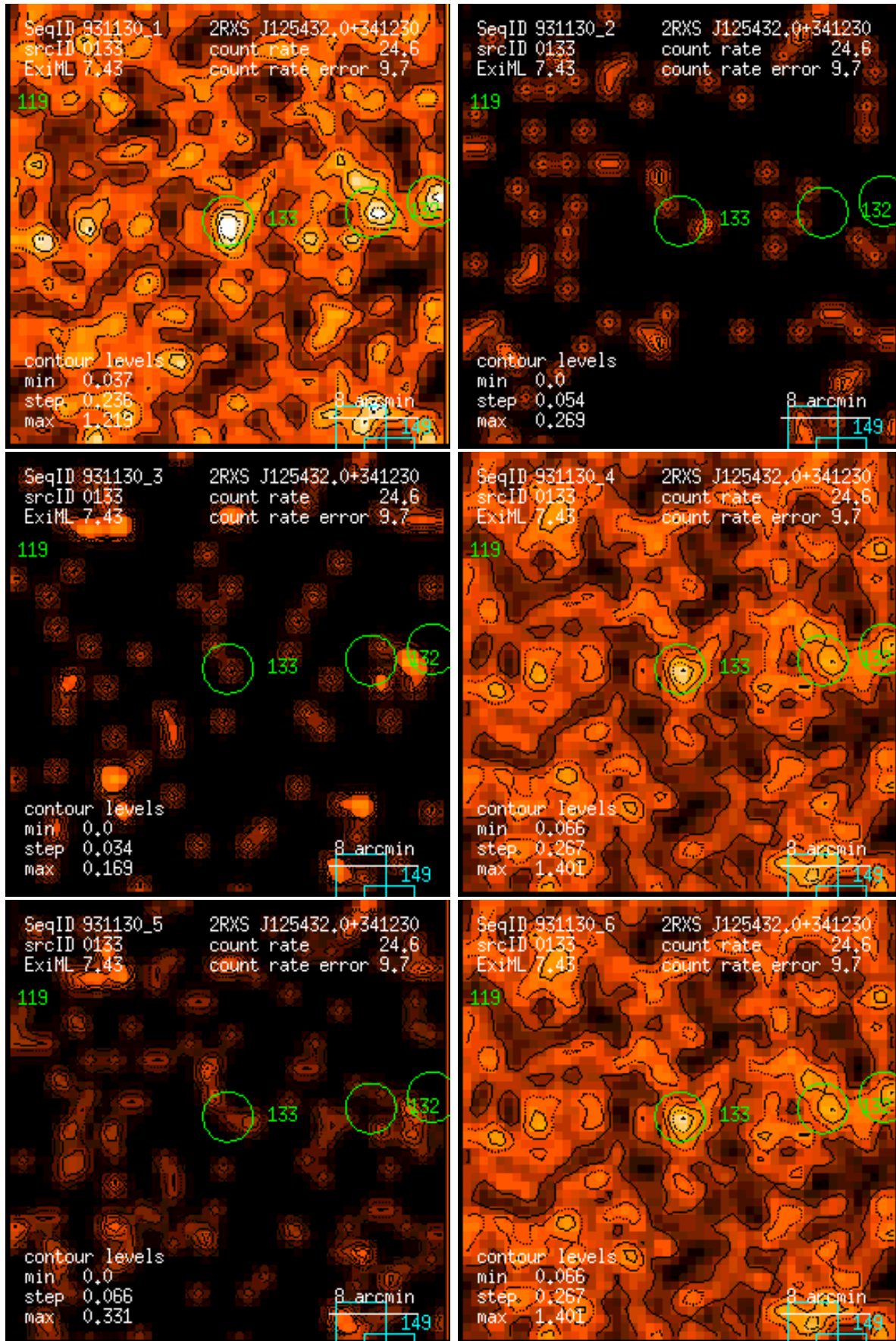
Figure 133: RASS 931130: detection 0133: band rate images, Gaussian filter: (1) PSPC channels 11 – 41, (2) 52 – 90, (3) 91 – 201, (4) 11 – 235, (5) 52 – 201, (6) 11 – 201. Broad band rates in counts/ks. Band rate contour levels in counts/ks/arcmin 2 .
