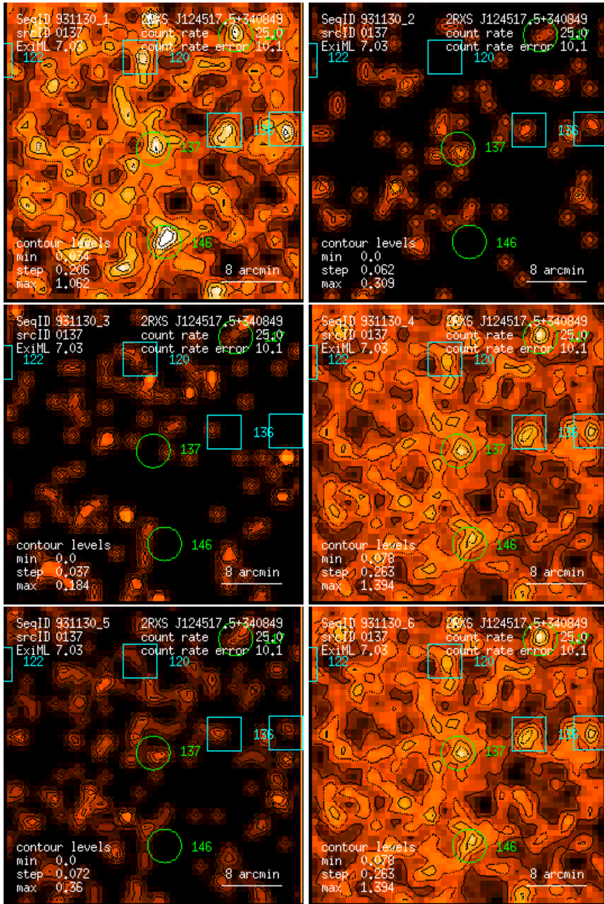
Figure 137: RASS 931130: detection 0137: band rate images, Gaussian filter: (1) PSPC channels 11 – 41, (2) 52 – 90, (3) 91 – 201, (4) 11 – 235, (5) 52 – 201, (6) 11 – 201. Broad band rates in counts/ks. Band rate contour levels in counts/ks/arcmin 2 .
