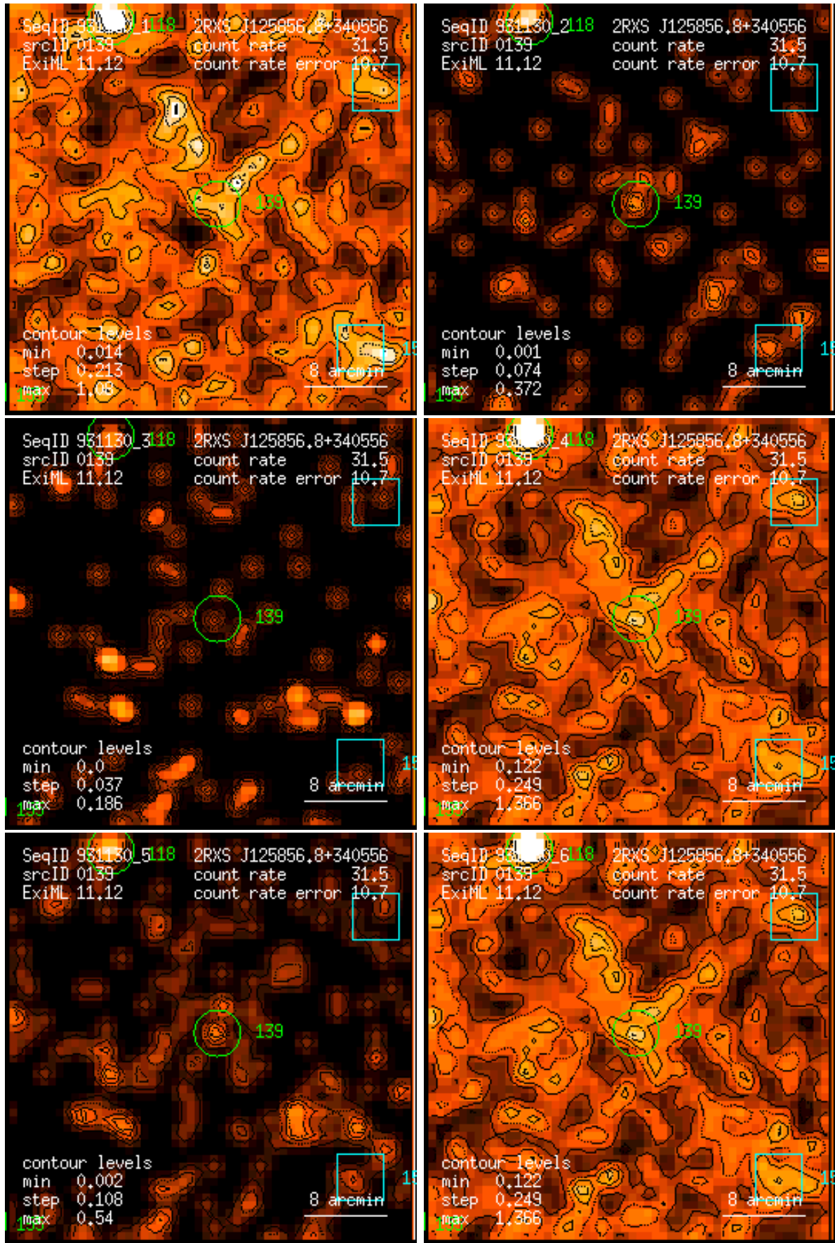
Figure 139: RASS 931130: detection 0139: band rate images, Gaussian filter: (1) PSPC channels 11 – 41, (2) 52 – 90, (3) 91 – 201, (4) 11 – 235, (5) 52 – 201, (6) 11 – 201. Broad band rates in counts/ks. Band rate contour levels in counts/ks/arcmin 2 .
