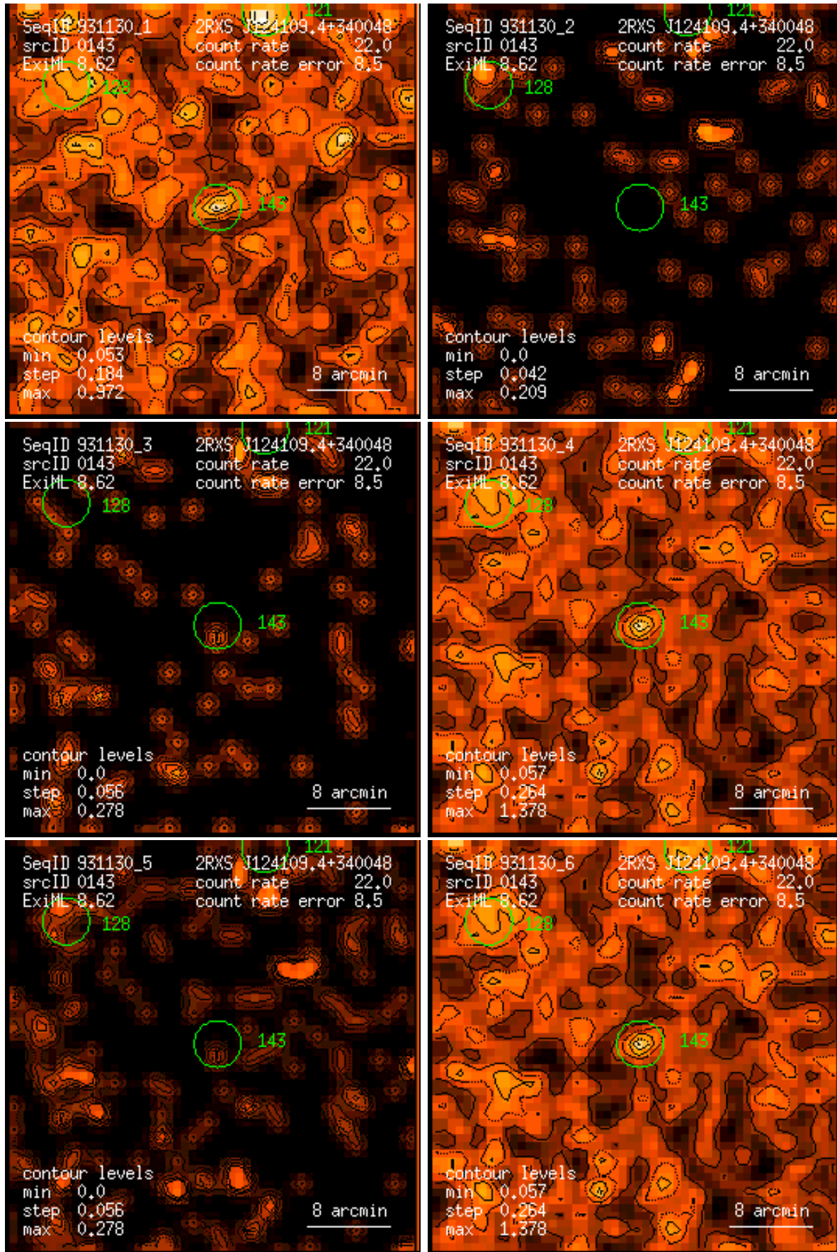
Figure 143: RASS 931130: detection 0143: band rate images, Gaussian filter: (1) PSPC channels 11 – 41, (2) 52 – 90, (3) 91 – 201, (4) 11 – 235, (5) 52 – 201, (6) 11 – 201. Broad band rates in counts/ks. Band rate contour levels in counts/ks/arcmin 2 .
