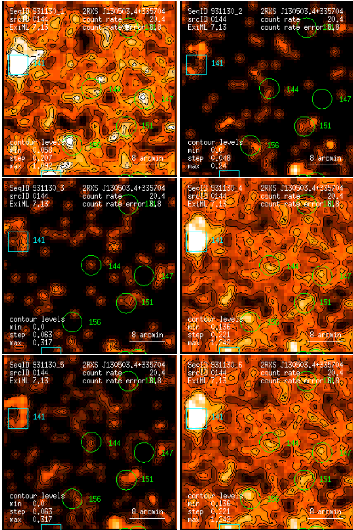
Figure 144: RASS 931130: detection 0144: band rate images, Gaussian filter: (1) PSPC channels 11 – 41, (2) 52 – 90, (3) 91 – 201, (4) 11 – 235, (5) 52 – 201, (6) 11 – 201. Broad band rates in counts/ks. Band rate contour levels in counts/ks/arcmin 2 .
