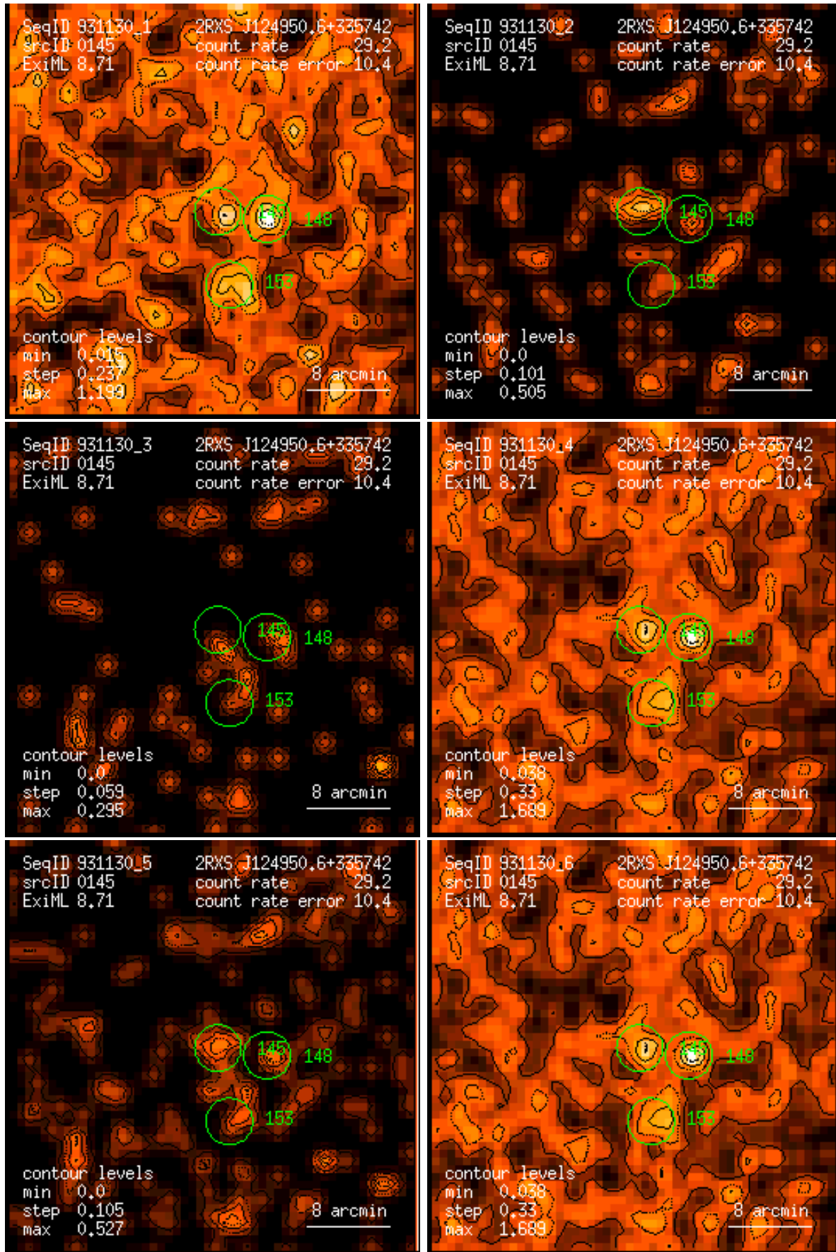
Figure 145: RASS 931130: detection 0145: band rate images, Gaussian filter: (1) PSPC channels 11 – 41, (2) 52 – 90, (3) 91 – 201, (4) 11 – 235, (5) 52 – 201, (6) 11 – 201. Broad band rates in counts/ks. Band rate contour levels in counts/ks/arcmin 2 .
