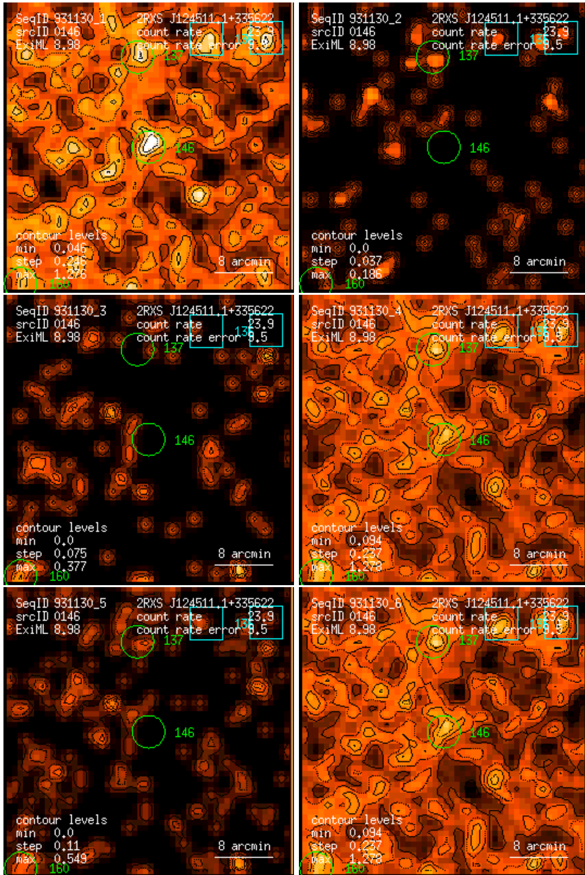
Figure 146: RASS 931130: detection 0146: band rate images, Gaussian filter: (1) PSPC channels 11 – 41, (2) 52 – 90, (3) 91 – 201, (4) 11 – 235, (5) 52 – 201, (6) 11 – 201. Broad band rates in counts/ks. Band rate contour levels in counts/ks/arcmin 2 .
