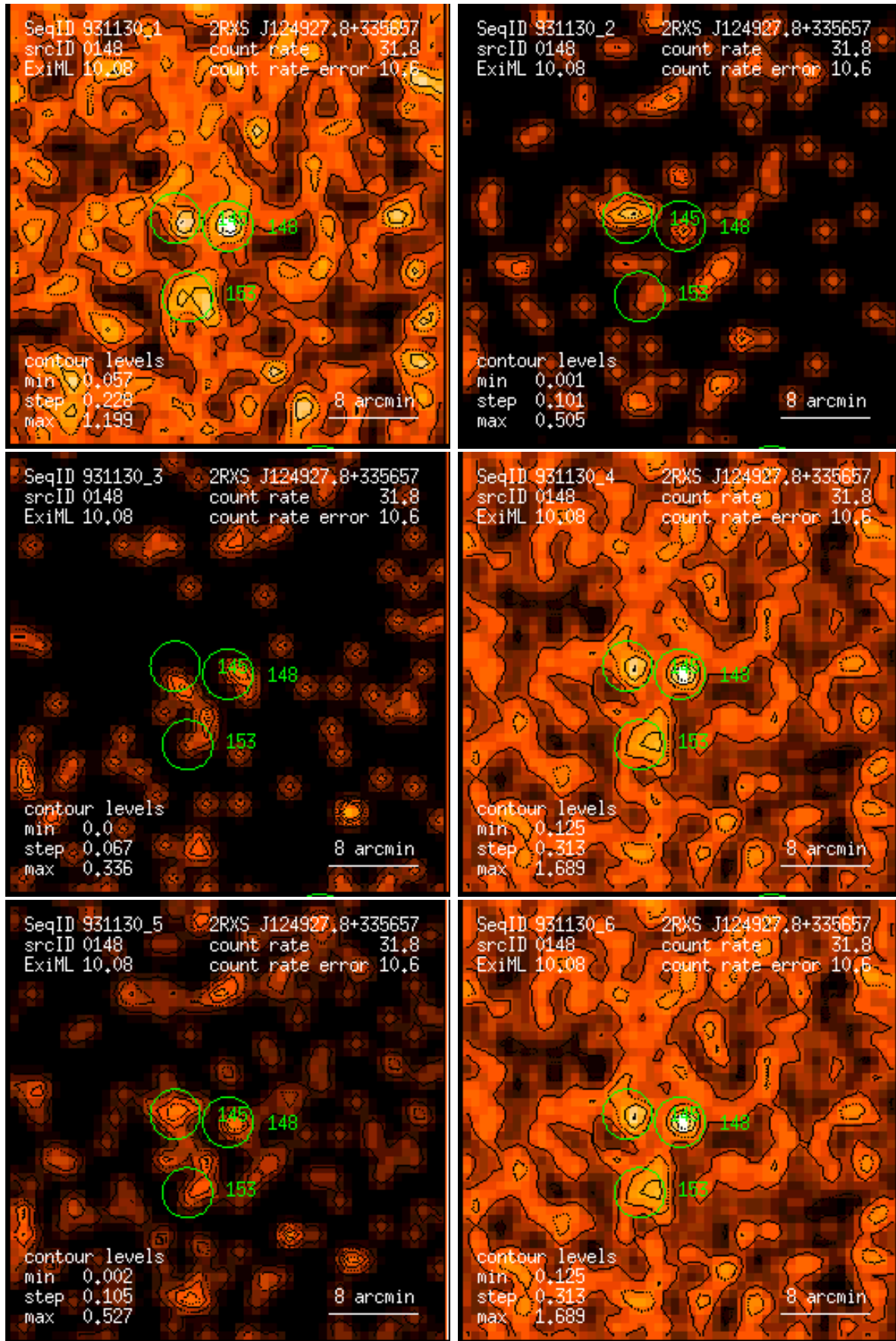
Figure 148: RASS 931130: detection 0148: band rate images, Gaussian filter: (1) PSPC channels 11 – 41, (2) 52 – 90, (3) 91 – 201, (4) 11 – 235, (5) 52 – 201, (6) 11 – 201. Broad band rates in counts/ks. Band rate contour levels in counts/ks/arcmin 2 .
