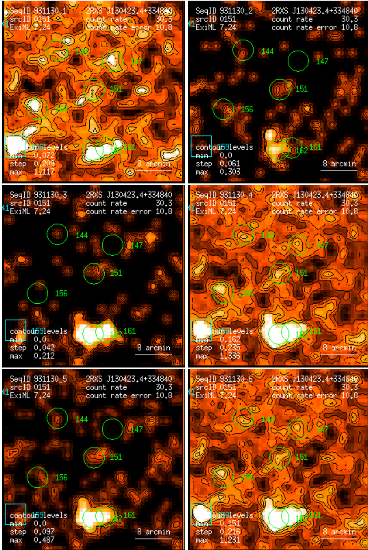
Figure 151: RASS 931130: detection 0151: band rate images, Gaussian filter: (1) PSPC channels 11 – 41, (2) 52 – 90, (3) 91 – 201, (4) 11 – 235, (5) 52 – 201, (6) 11 – 201. Broad band rates in counts/ks. Band rate contour levels in counts/ks/arcmin 2 .
