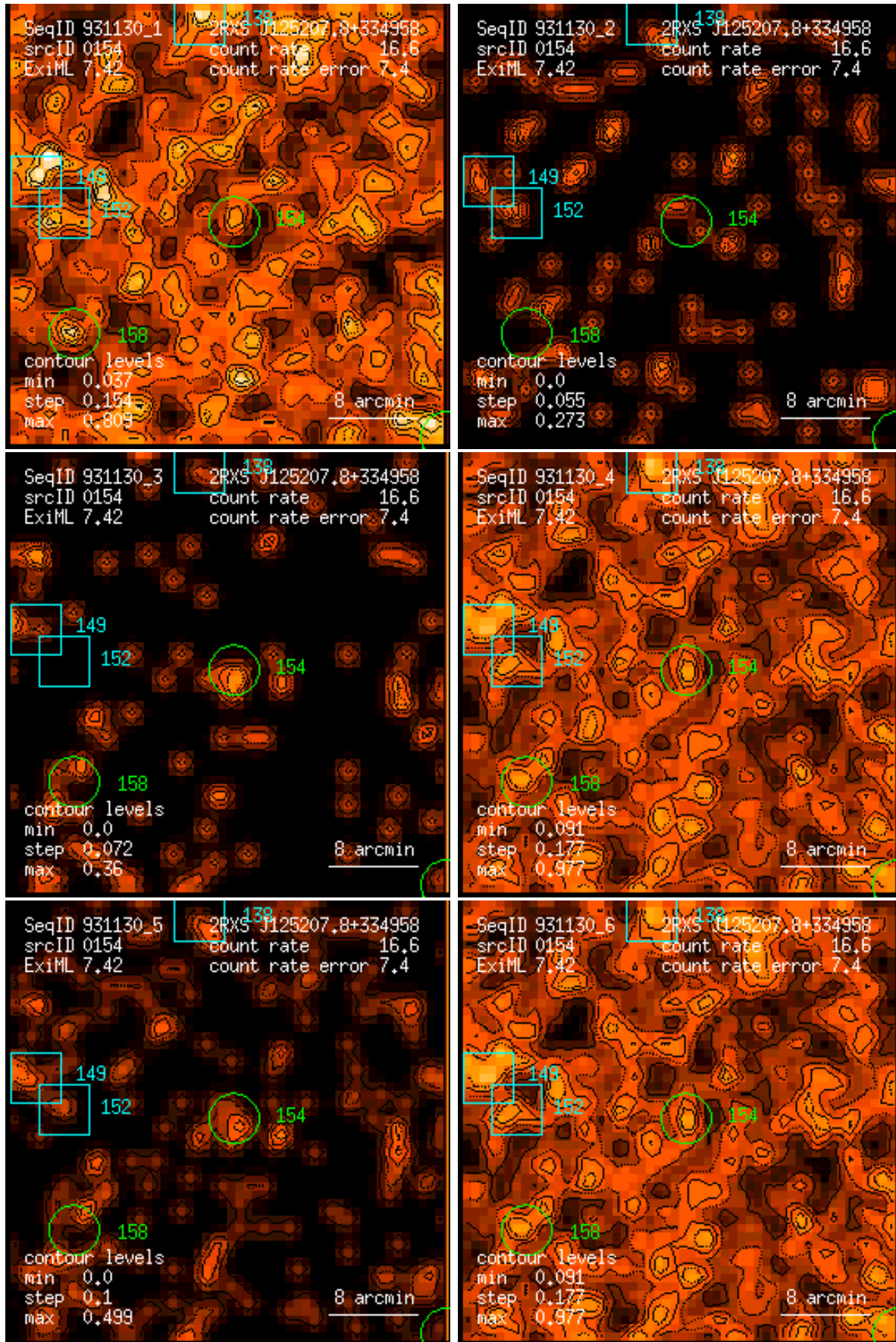
Figure 154: RASS 931130: detection 0154: band rate images, Gaussian filter: (1) PSPC channels 11 – 41, (2) 52 – 90, (3) 91 – 201, (4) 11 – 235, (5) 52 – 201, (6) 11 – 201. Broad band rates in counts/ks. Band rate contour levels in counts/ks/arcmin 2 .
