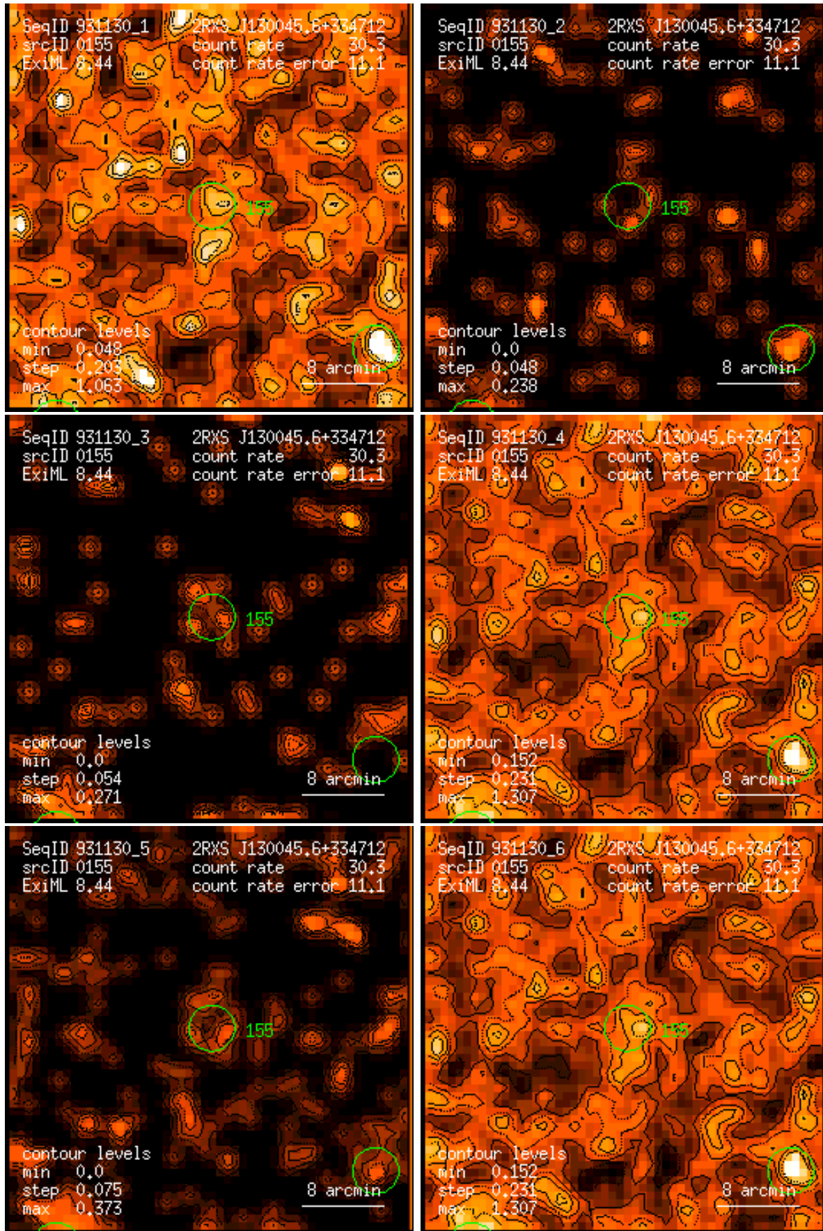
Figure 155: RASS 931130: detection 0155: band rate images, Gaussian filter: (1) PSPC channels 11 – 41, (2) 52 – 90, (3) 91 – 201, (4) 11 – 235, (5) 52 – 201, (6) 11 – 201. Broad band rates in counts/ks. Band rate contour levels in counts/ks/arcmin 2 .
