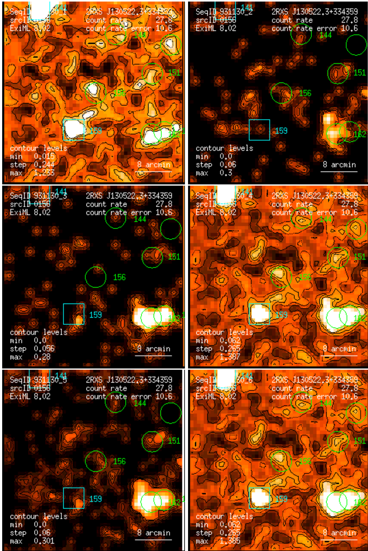
Figure 156: RASS 931130: detection 0156: band rate images, Gaussian filter: (1) PSPC channels 11 – 41, (2) 52 – 90, (3) 91 – 201, (4) 11 – 235, (5) 52 – 201, (6) 11 – 201. Broad band rates in counts/ks. Band rate contour levels in counts/ks/arcmin 2 .
