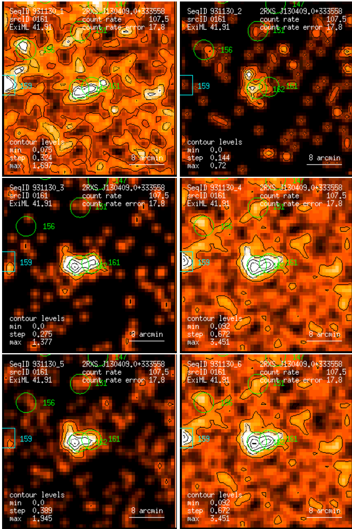
Figure 161: RASS 931130: detection 0161: band rate images, Gaussian filter: (1) PSPC channels 11 – 41, (2) 52 – 90, (3) 91 – 201, (4) 11 – 235, (5) 52 – 201, (6) 11 – 201. Broad band rates in counts/ks. Band rate contour levels in counts/ks/arcmin 2 .
