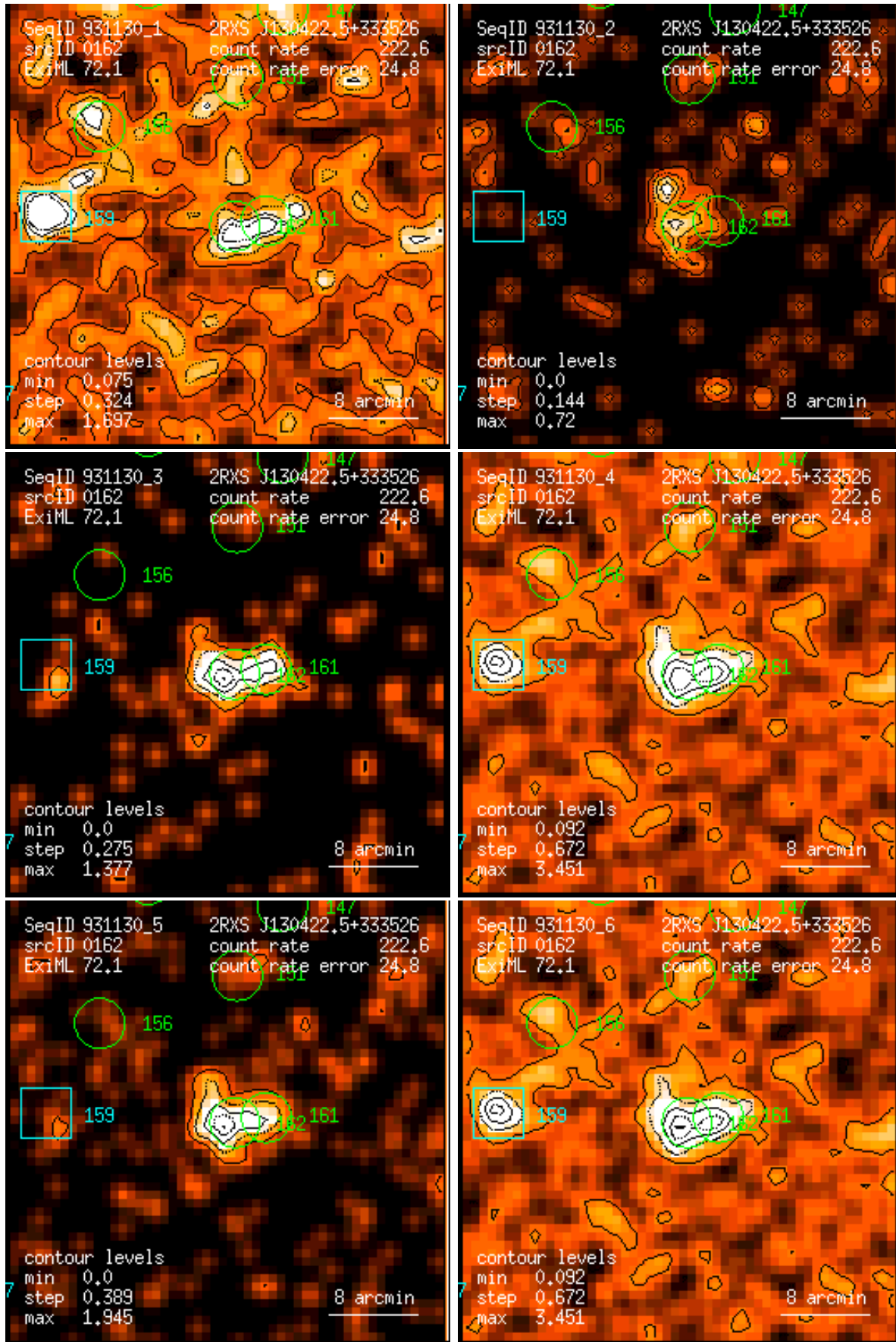
Figure 162: RASS 931130: detection 0162: band rate images, Gaussian filter: (1) PSPC channels 11 – 41, (2) 52 – 90, (3) 91 – 201, (4) 11 – 235, (5) 52 – 201, (6) 11 – 201. Broad band rates in counts/ks. Band rate contour levels in counts/ks/arcmin 2 .
