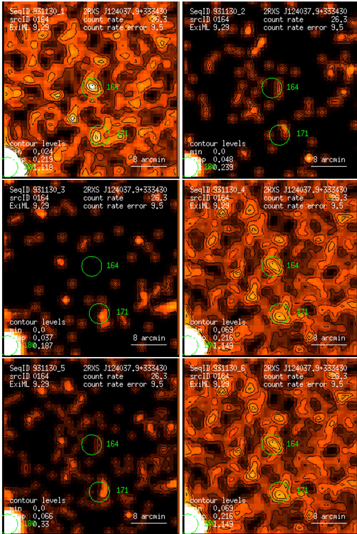
Figure 164: RASS 931130: detection 0164: band rate images, Gaussian filter: (1) PSPC channels 11 – 41, (2) 52 – 90, (3) 91 – 201, (4) 11 – 235, (5) 52 – 201, (6) 11 – 201. Broad band rates in counts/ks. Band rate contour levels in counts/ks/arcmin 2 .
