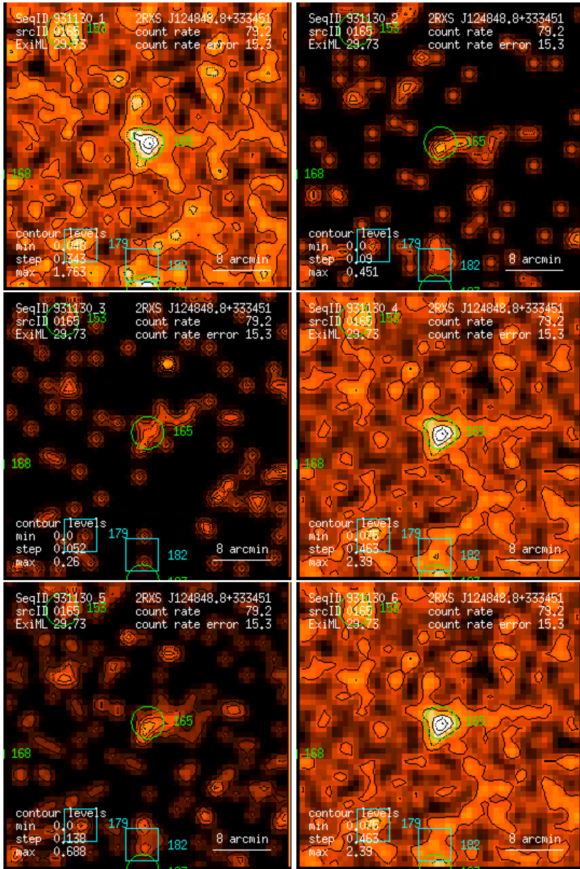
Figure 165: RASS 931130: detection 0165: band rate images, Gaussian filter: (1) PSPC channels 11 – 41, (2) 52 – 90, (3) 91 – 201, (4) 11 – 235, (5) 52 – 201, (6) 11 – 201. Broad band rates in counts/ks. Band rate contour levels in counts/ks/arcmin 2 .
