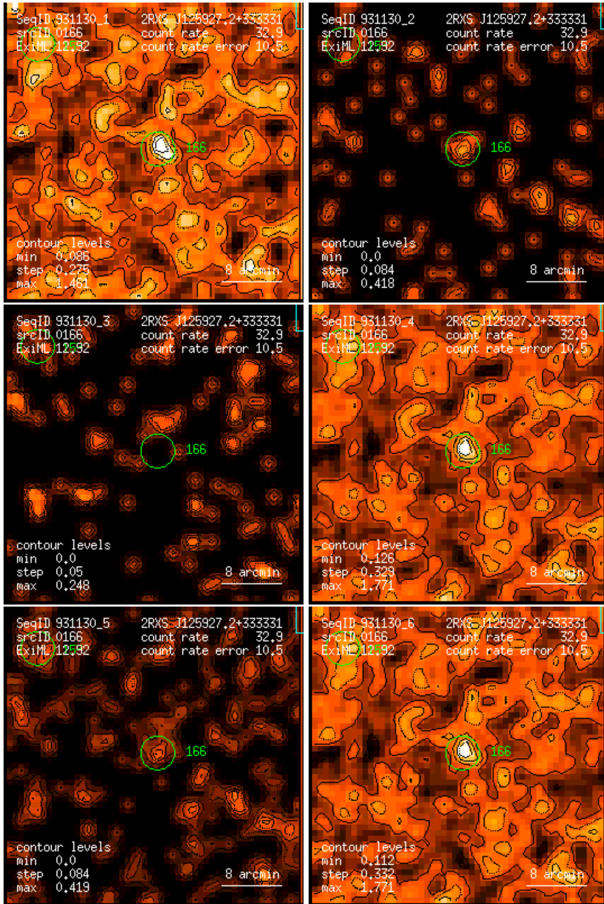
Figure 166: RASS 931130: detection 0166: band rate images, Gaussian filter: (1) PSPC channels 11 – 41, (2) 52 – 90, (3) 91 – 201, (4) 11 – 235, (5) 52 – 201, (6) 11 – 201. Broad band rates in counts/ks. Band rate contour levels in counts/ks/arcmin 2 .
