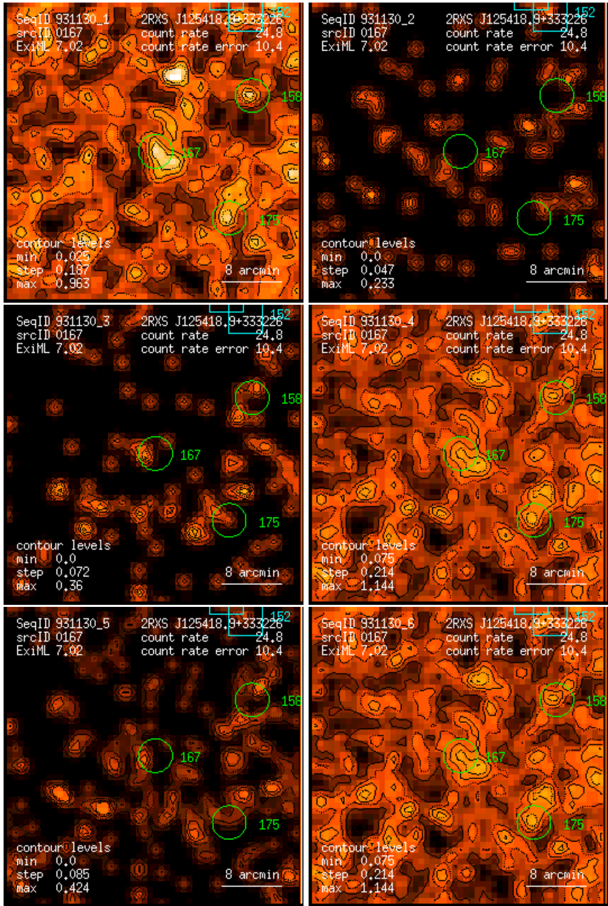
Figure 167: RASS 931130: detection 0167: band rate images, Gaussian filter: (1) PSPC channels 11 – 41, (2) 52 – 90, (3) 91 – 201, (4) 11 – 235, (5) 52 – 201, (6) 11 – 201. Broad band rates in counts/ks. Band rate contour levels in counts/ks/arcmin 2 .
