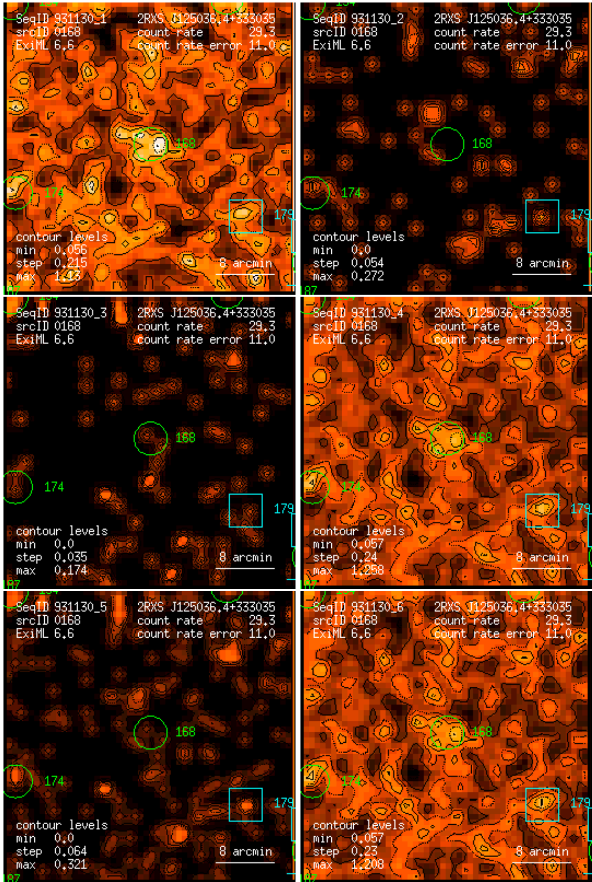
Figure 168: RASS 931130: detection 0168: band rate images, Gaussian filter: (1) PSPC channels 11 – 41, (2) 52 – 90, (3) 91 – 201, (4) 11 – 235, (5) 52 – 201, (6) 11 – 201. Broad band rates in counts/ks. Band rate contour levels in counts/ks/arcmin 2 .
