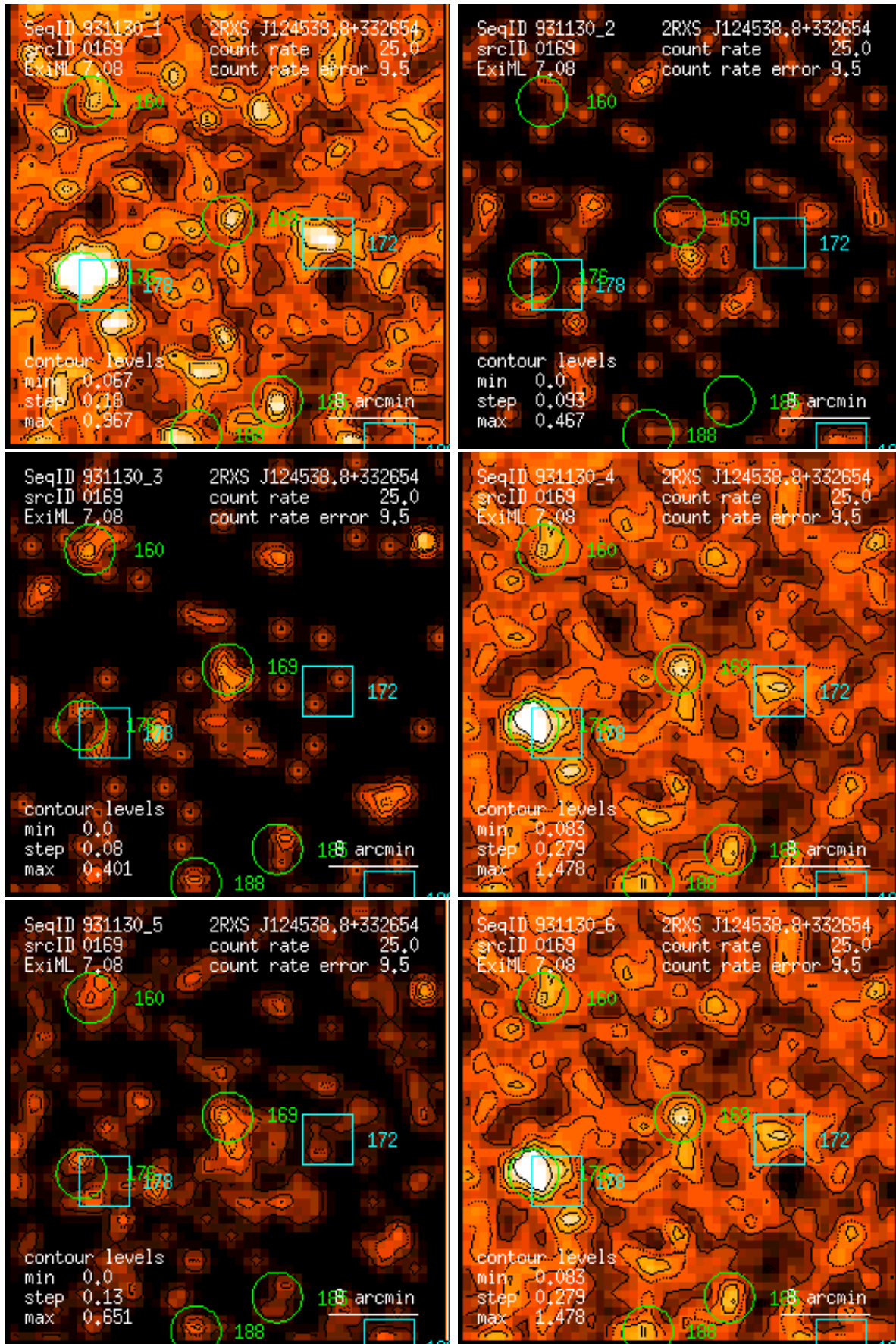
Figure 169: RASS 931130: detection 0169: band rate images, Gaussian filter: (1) PSPC channels 11 – 41, (2) 52 – 90, (3) 91 – 201, (4) 11 – 235, (5) 52 – 201, (6) 11 – 201. Broad band rates in counts/ks. Band rate contour levels in counts/ks/arcmin 2 .
