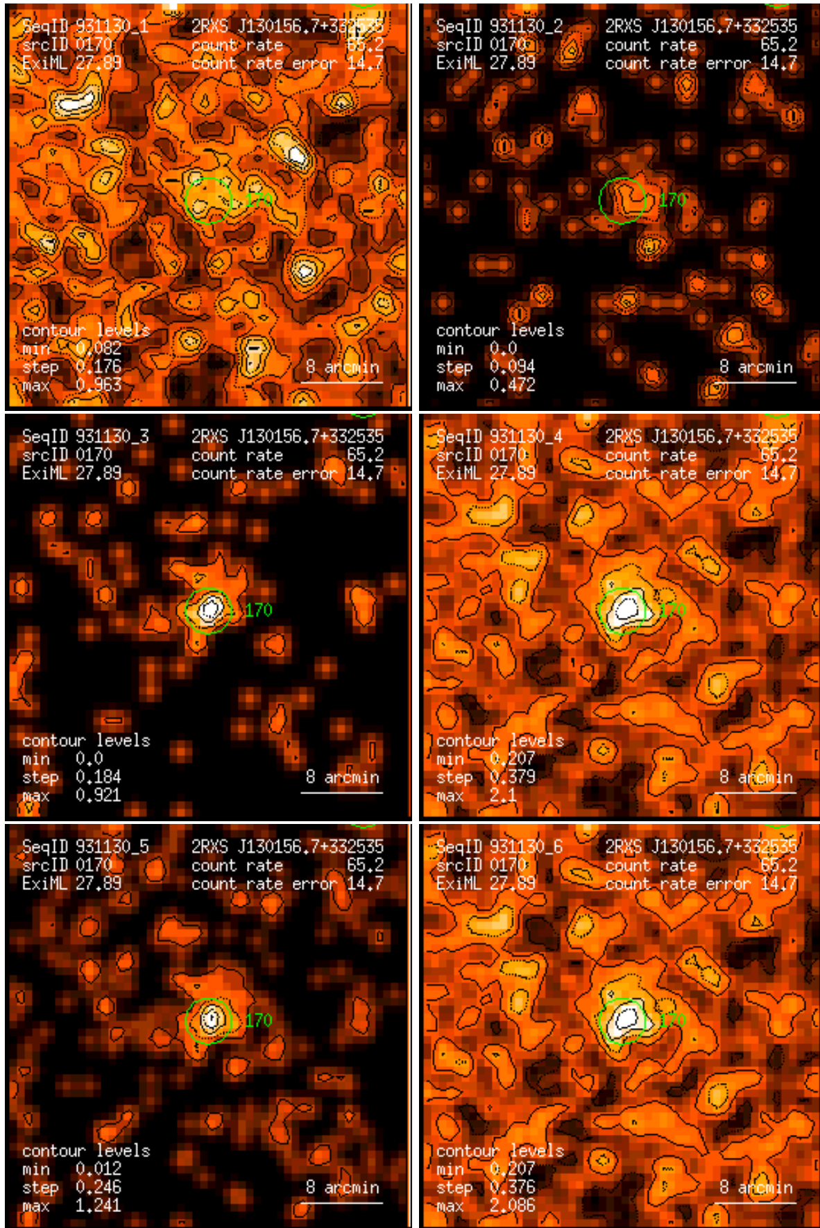
Figure 170: RASS 931130: detection 0170: band rate images, Gaussian filter: (1) PSPC channels 11 – 41, (2) 52 – 90, (3) 91 – 201, (4) 11 – 235, (5) 52 – 201, (6) 11 – 201. Broad band rates in counts/ks. Band rate contour levels in counts/ks/arcmin 2 .
