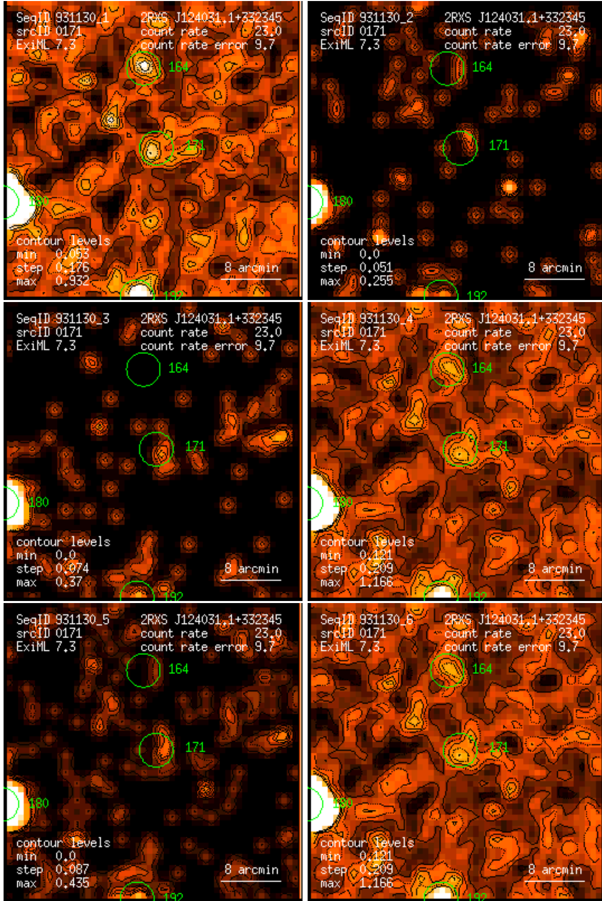
Figure 171: RASS 931130: detection 0171: band rate images, Gaussian filter: (1) PSPC channels 11 – 41, (2) 52 – 90, (3) 91 – 201, (4) 11 – 235, (5) 52 – 201, (6) 11 – 201. Broad band rates in counts/ks. Band rate contour levels in counts/ks/arcmin 2 .
