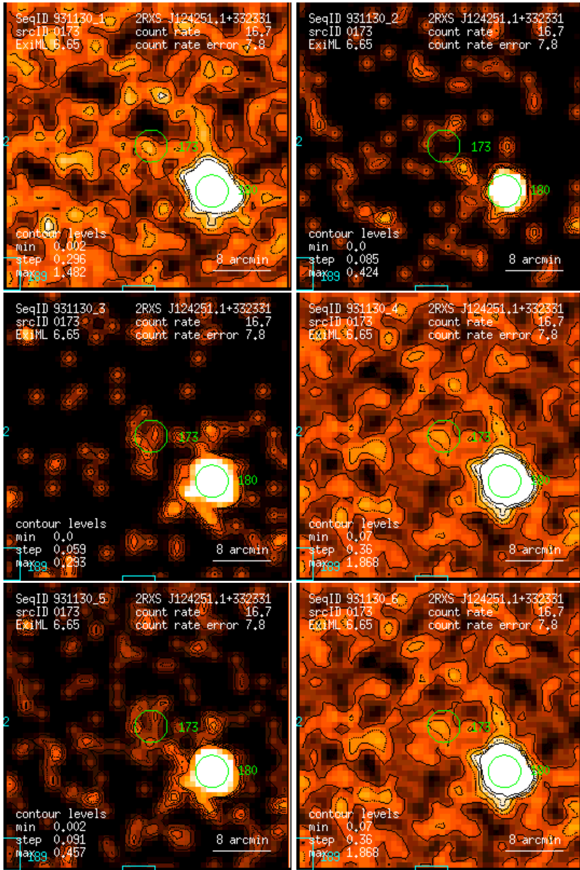
Figure 173: RASS 931130: detection 0173: band rate images, Gaussian filter: (1) PSPC channels 11 – 41, (2) 52 – 90, (3) 91 – 201, (4) 11 – 235, (5) 52 – 201, (6) 11 – 201. Broad band rates in counts/ks. Band rate contour levels in counts/ks/arcmin 2 .
