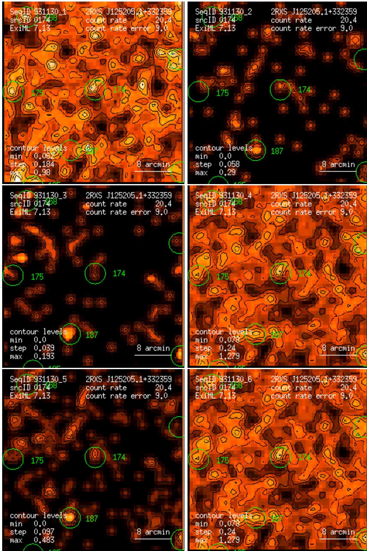
Figure 174: RASS 931130: detection 0174: band rate images, Gaussian filter: (1) PSPC channels 11 – 41, (2) 52 – 90, (3) 91 – 201, (4) 11 – 235, (5) 52 – 201, (6) 11 – 201. Broad band rates in counts/ks. Band rate contour levels in counts/ks/arcmin 2 .
