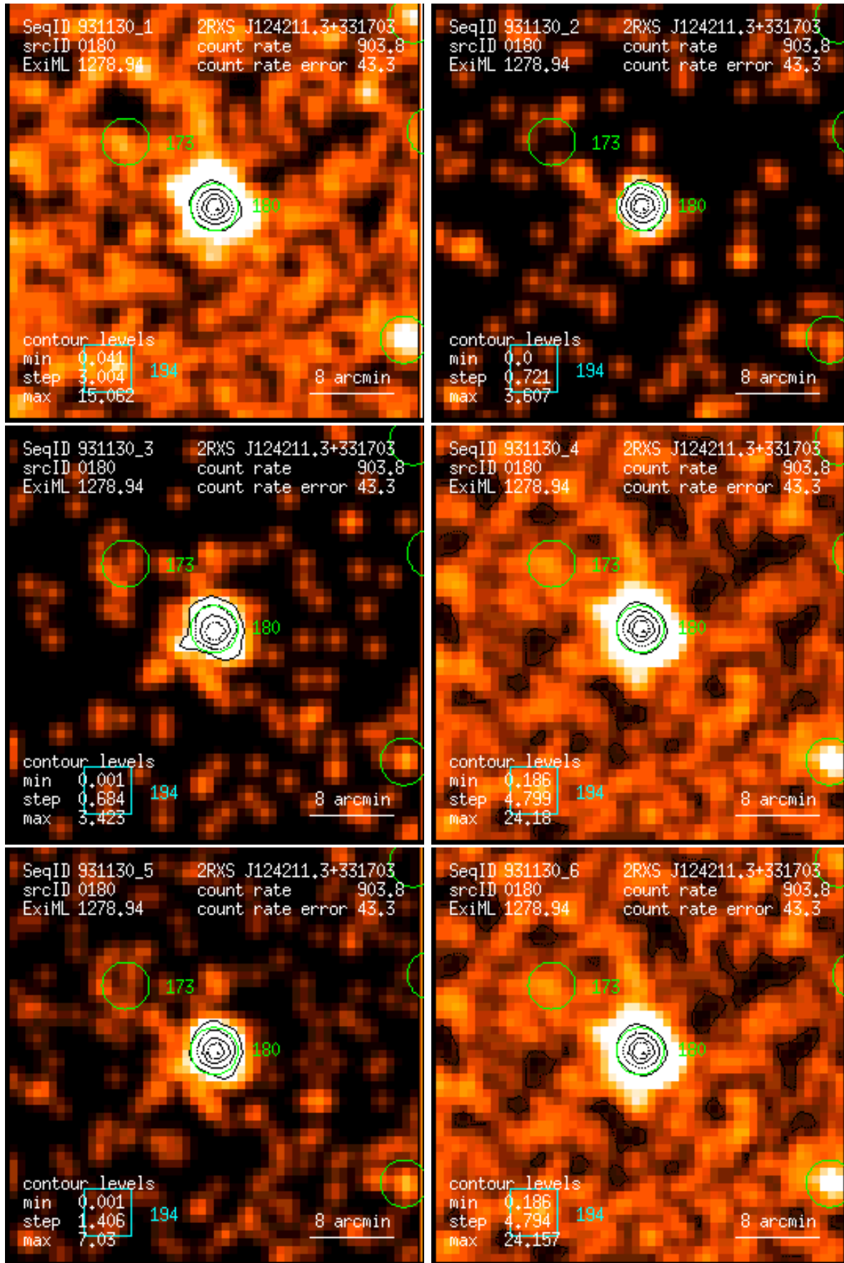
Figure 180: RASS 931130: detection 0180: band rate images, Gaussian filter: (1) PSPC channels 11 – 41, (2) 52 – 90, (3) 91 – 201, (4) 11 – 235, (5) 52 – 201, (6) 11 – 201. Broad band rates in counts/ks. Band rate contour levels in counts/ks/arcmin 2 .
