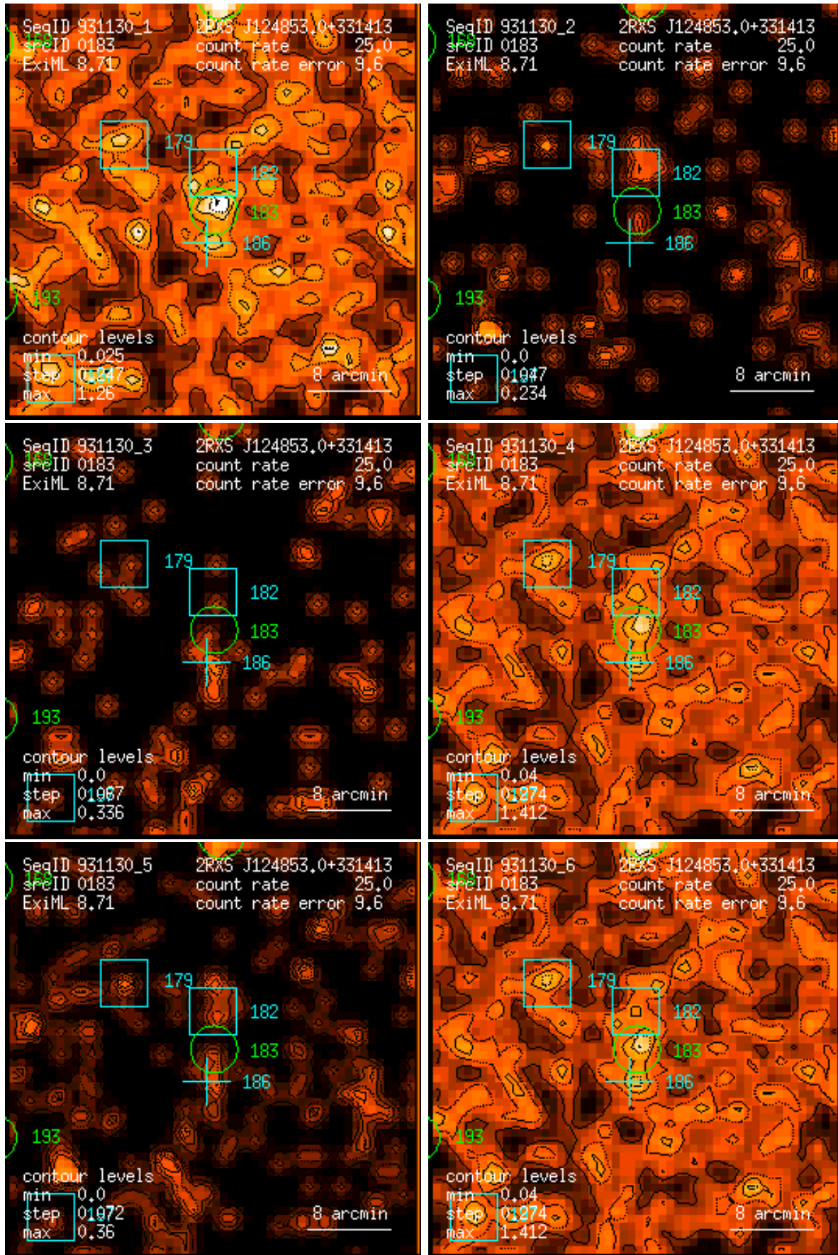
Figure 183: RASS 931130: detection 0183: band rate images, Gaussian filter: (1) PSPC channels 11 – 41, (2) 52 – 90, (3) 91 – 201, (4) 11 – 235, (5) 52 – 201, (6) 11 – 201. Broad band rates in counts/ks. Band rate contour levels in counts/ks/arcmin 2 .
