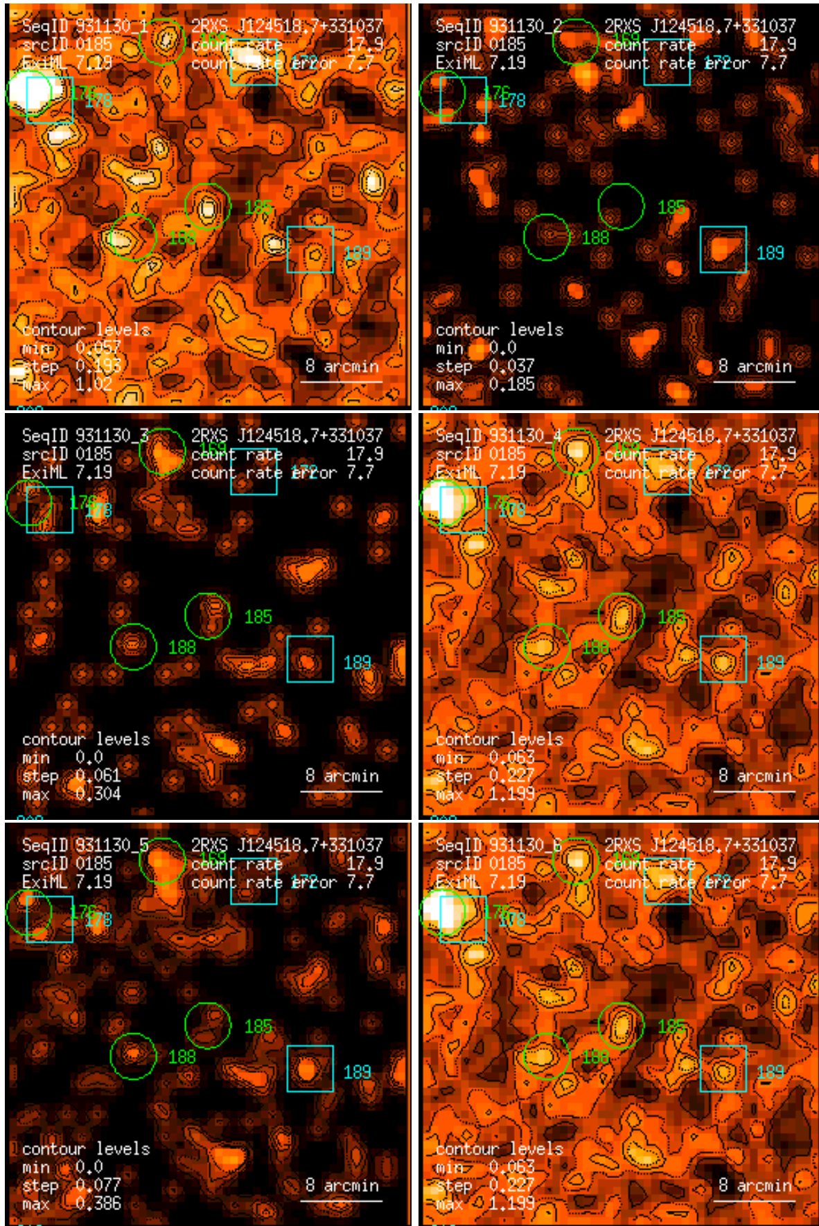
Figure 185: RASS 931130: detection 0185: band rate images, Gaussian filter: (1) PSPC channels 11 – 41, (2) 52 – 90, (3) 91 – 201, (4) 11 – 235, (5) 52 – 201, (6) 11 – 201. Broad band rates in counts/ks. Band rate contour levels in counts/ks/arcmin 2 .
