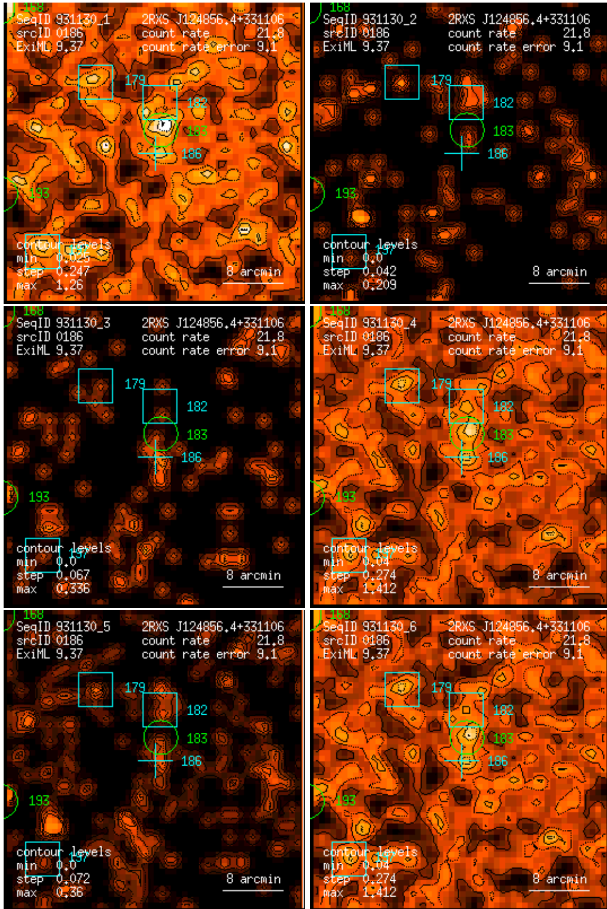
Figure 186: RASS 931130: detection 0186: band rate images, Gaussian filter: (1) PSPC channels 11 – 41, (2) 52 – 90, (3) 91 – 201, (4) 11 – 235, (5) 52 – 201, (6) 11 – 201. Broad band rates in counts/ks. Band rate contour levels in counts/ks/arcmin 2 .
