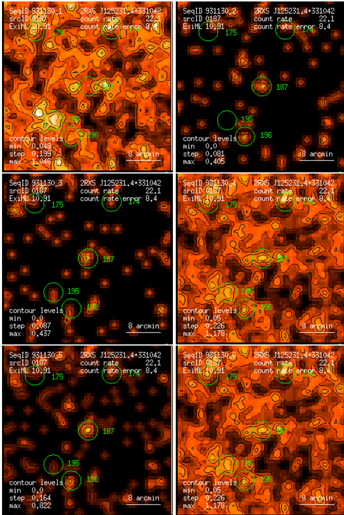
Figure 187: RASS 931130: detection 0187: band rate images, Gaussian filter: (1) PSPC channels 11 – 41, (2) 52 – 90, (3) 91 – 201, (4) 11 – 235, (5) 52 – 201, (6) 11 – 201. Broad band rates in counts/ks. Band rate contour levels in counts/ks/arcmin 2 .
