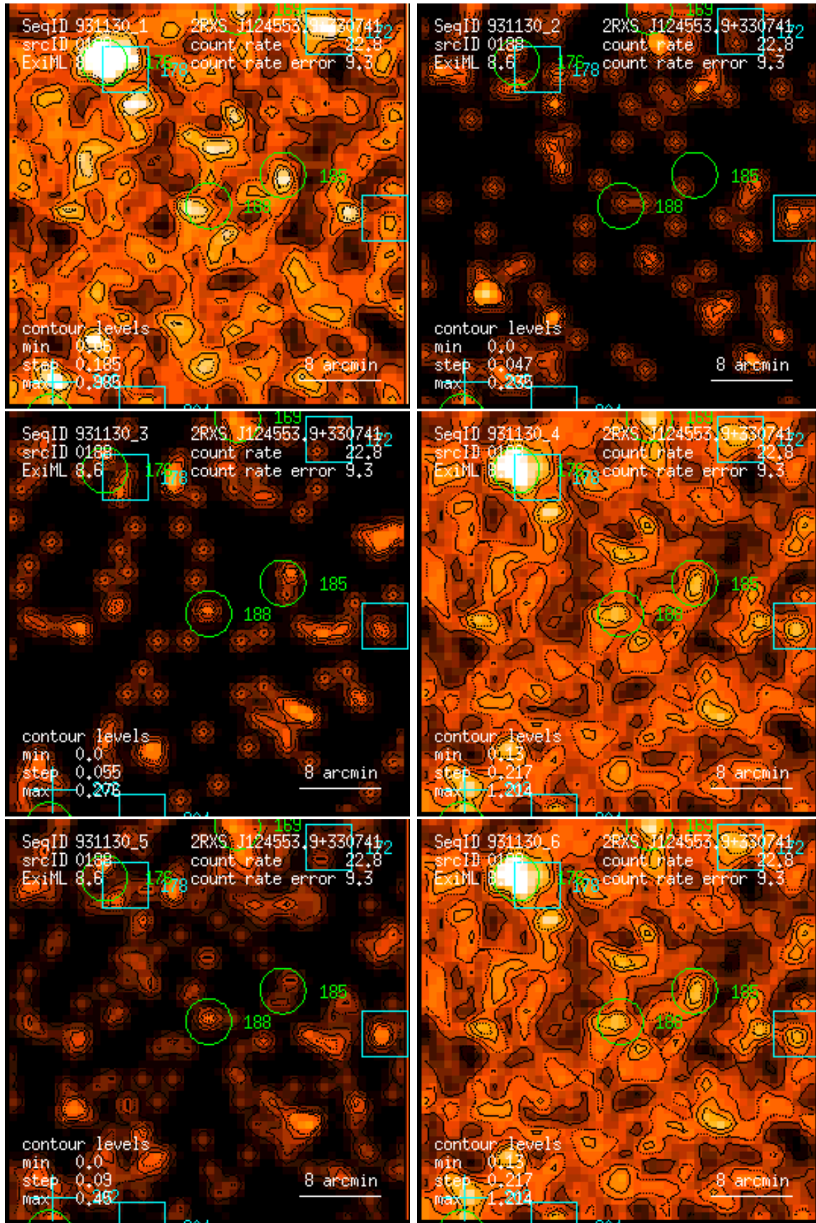
Figure 188: RASS 931130: detection 0188: band rate images, Gaussian filter: (1) PSPC channels 11 – 41, (2) 52 – 90, (3) 91 – 201, (4) 11 – 235, (5) 52 – 201, (6) 11 – 201. Broad band rates in counts/ks. Band rate contour levels in counts/ks/arcmin 2 .
